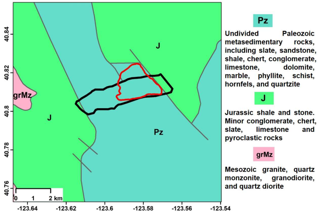
Figure S1. Geologic units of the study area modified from geological map of California (2010). The gray lines show the faults. It should be noted that the geologic terrane boundaries on this map are also faults.
