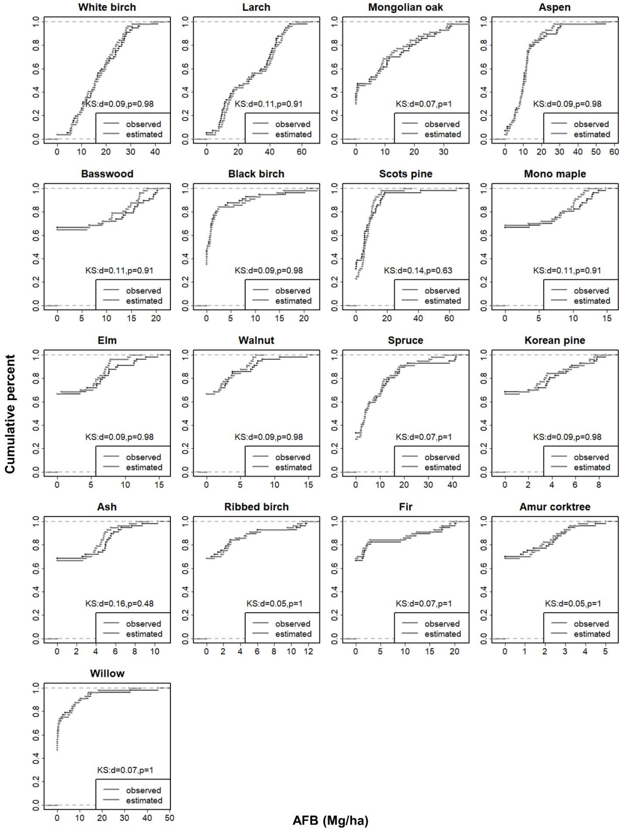
Figure S4. Cumulative distribution functions of the observed and the estimated AFB for 17 species separately based on the testing data at the ecotype level.
