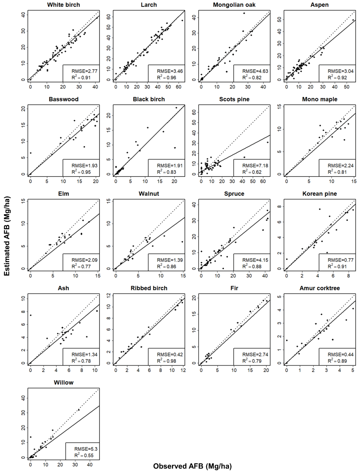
Figure S3. Scatter plot between the observed and the estimated AFB for 17 species separately based on the testing data at the ecotype level. Note that the dotted line is the 1:1 line.
