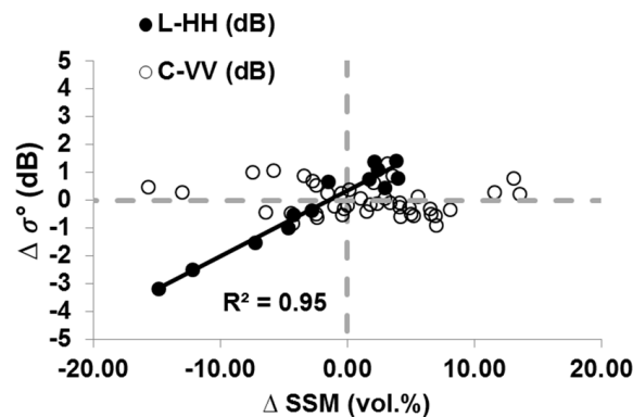
Figure 5. \Delta \sigma^0 (difference in \sigma^0 between two successive dates) in the L and C bands versus \Delta \text{SSM} (corresponding difference of SSM) for reference plots of wheat and grassland with an NDVI greater than 0.7. Positive \Delta \sigma^0 and \Delta \text{SSM} correspond to increases between two successive dates of \sigma^0 and SSM, respectively.
