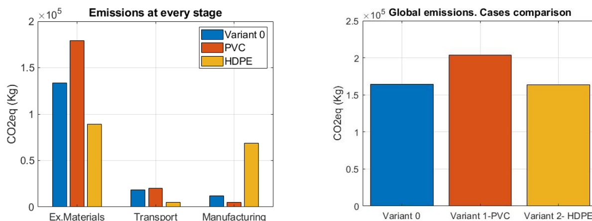
Figure 3. Variants comparison for “cradle-to-gate” system boundary.
