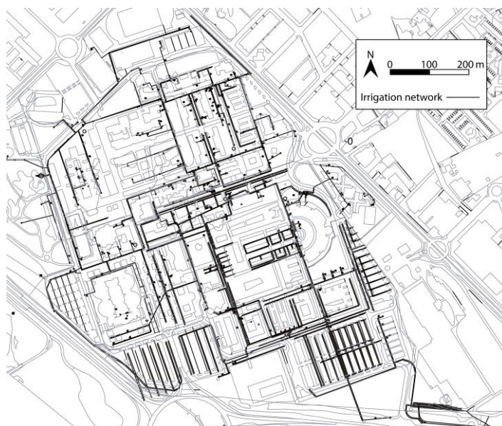
Figure 2. Looped irrigation network of the University of Alicante.
