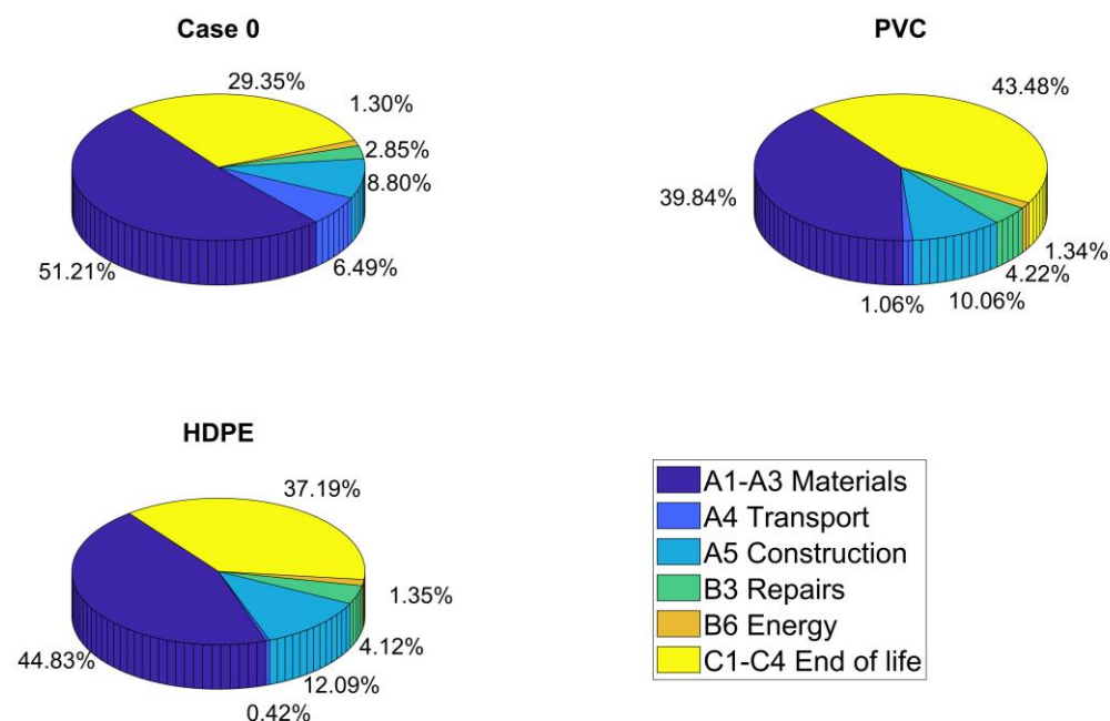
Figure 4. Percentage share of life cycle stages on total CO 2e emissions for 25 years.
