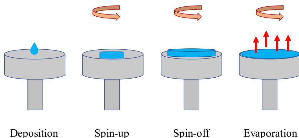
Figure 3. Spin coating process.
