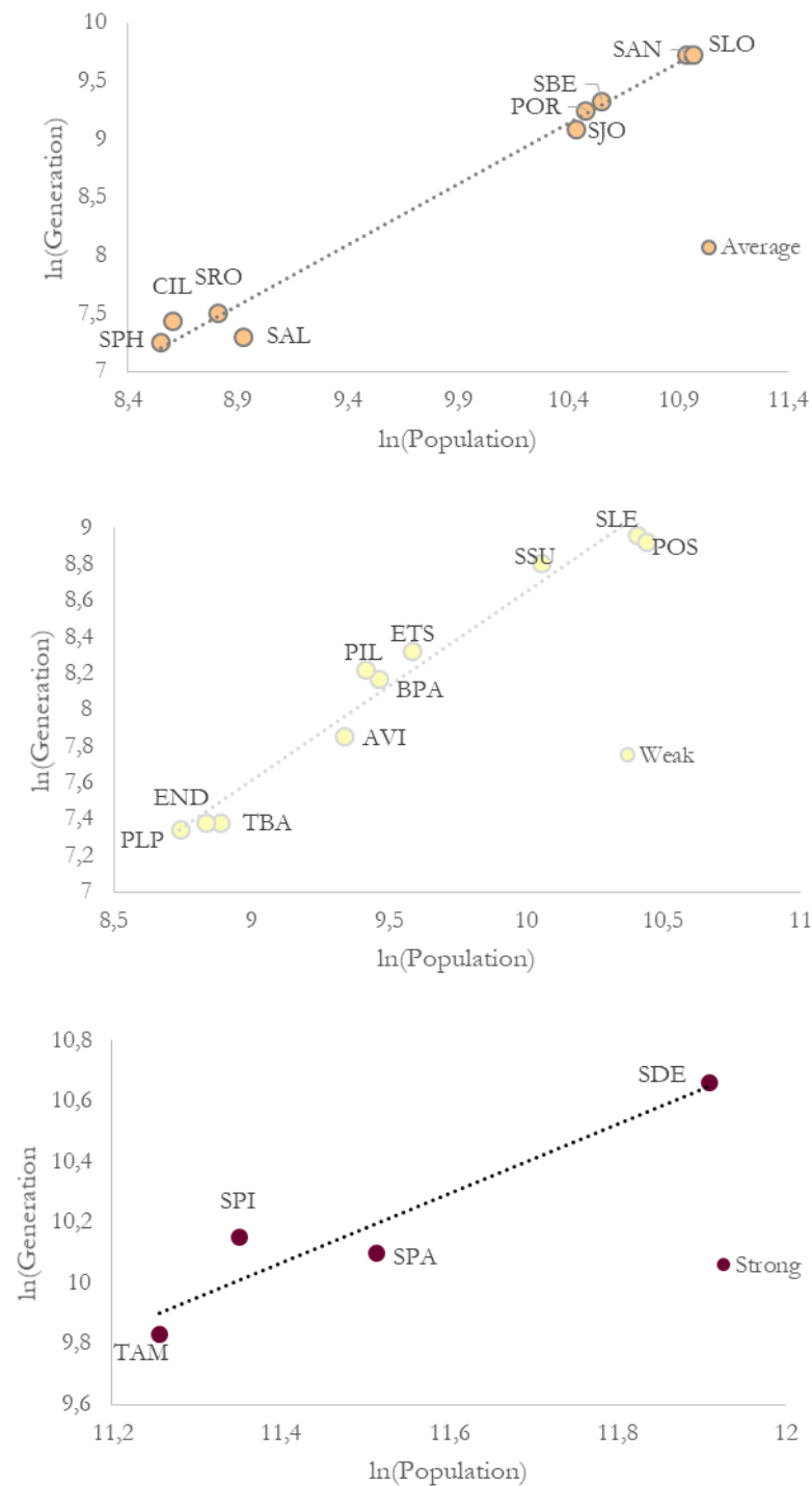
Figure 10. Linear regression model R2—population/waste generation.
