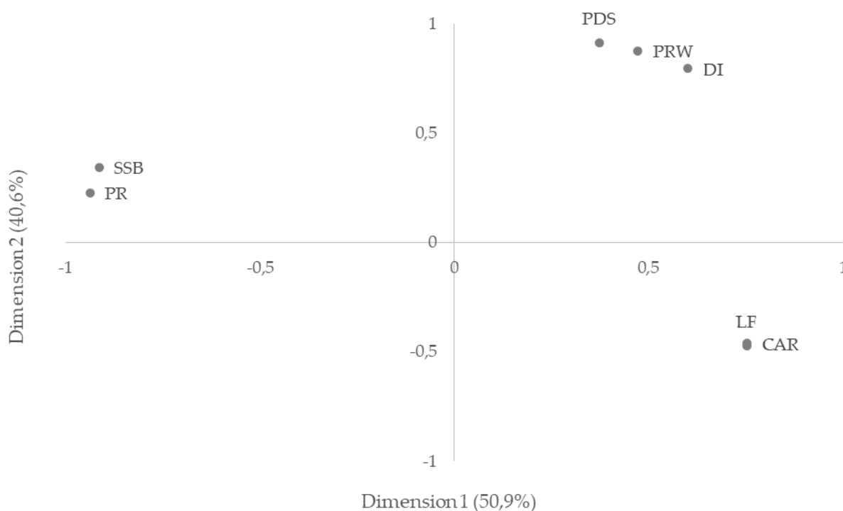
Figure 8. Graph of the variables.
