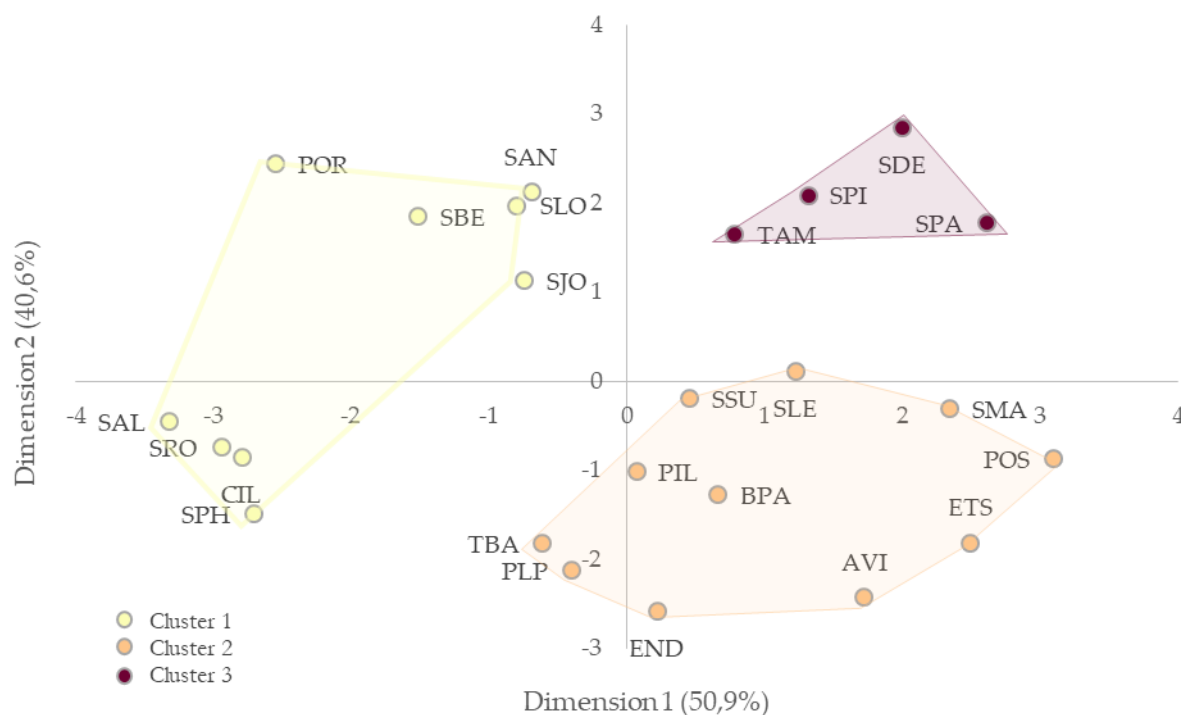
Figure 9. Graph of the individuals.
