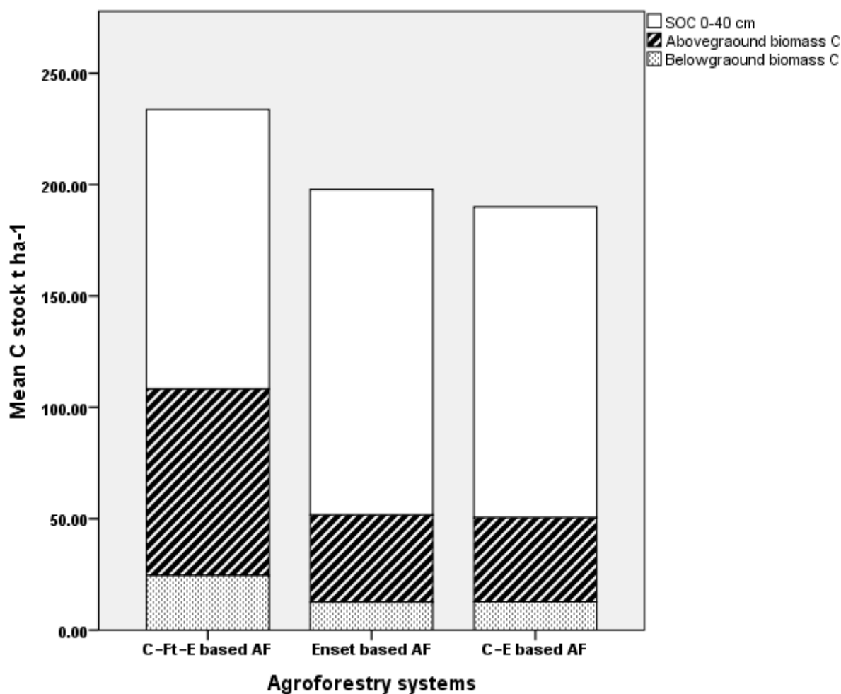
Figure 6. Agroforestry total carbon stocks (including trees, shrubs, coffee, enset, stumps, and large roots, SOC 0–40 cm) ( \text{t ha}^{-1} ) by AF system.
