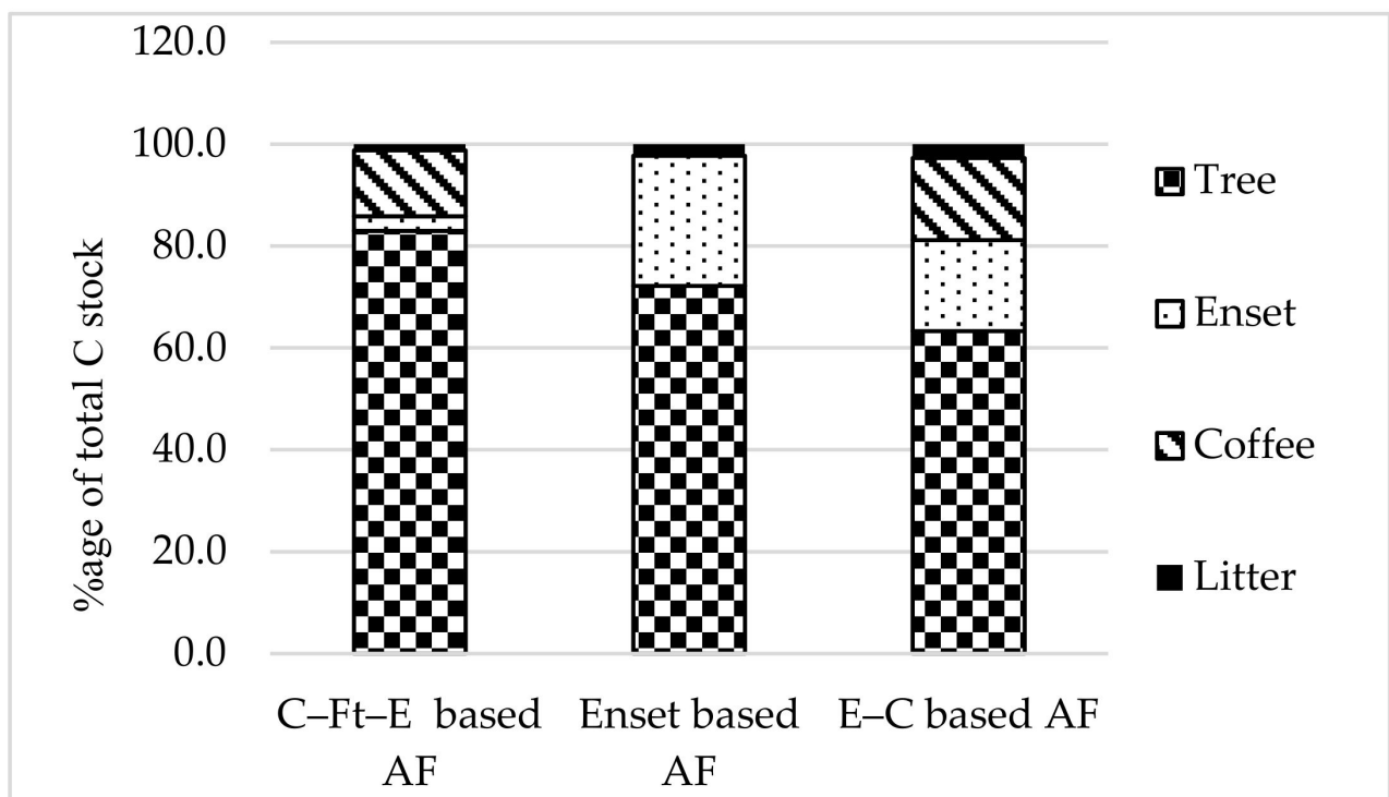
Figure 4. Proportion of C stock of each component in the aboveground biomass. C-Ft-E AF= Coffee-Fruit-tree-Enset based agroforestry; C-E based AF = Coffee-Enset based agroforestry.
