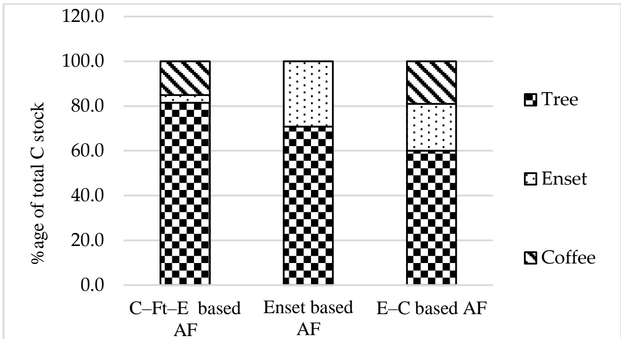
Figure 5. Proportion of carbon stock of each component in the belowground biomass. C-Ft-E AF= Coffee-Fruit-tree-Enset based agroforestry; C-E AF = Coffee-Enset based agroforestry.
