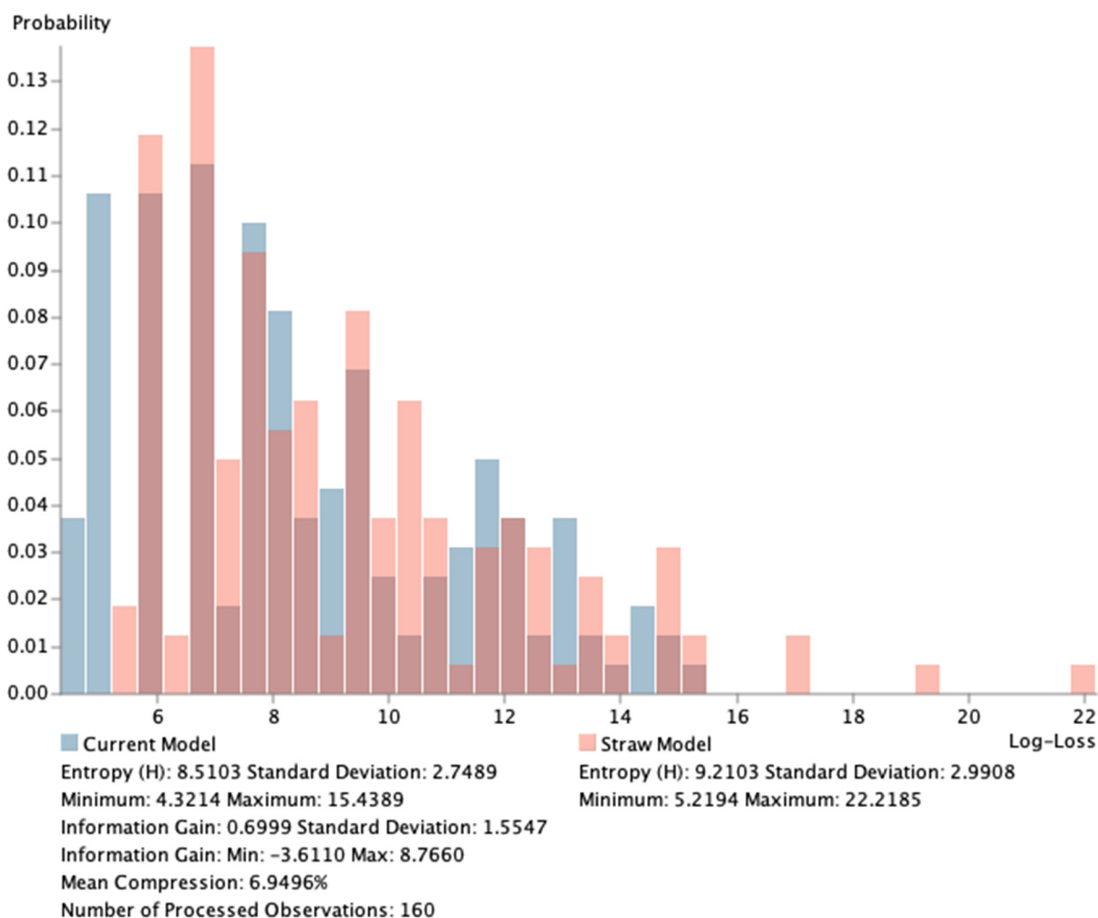
Figure 2. The BN network performance.
