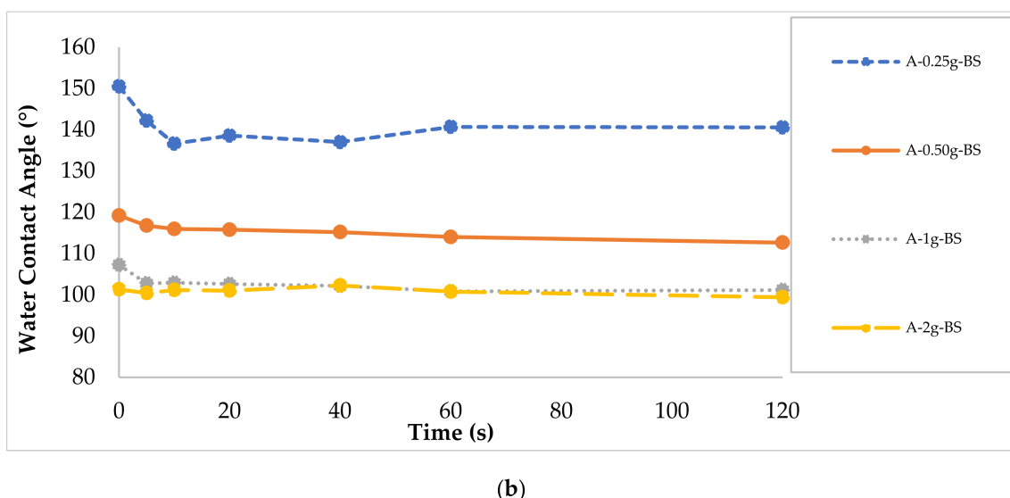
Figure 14. Results of water contact angle for Mixture A: (a) with resin, and (b) resin+BS.
