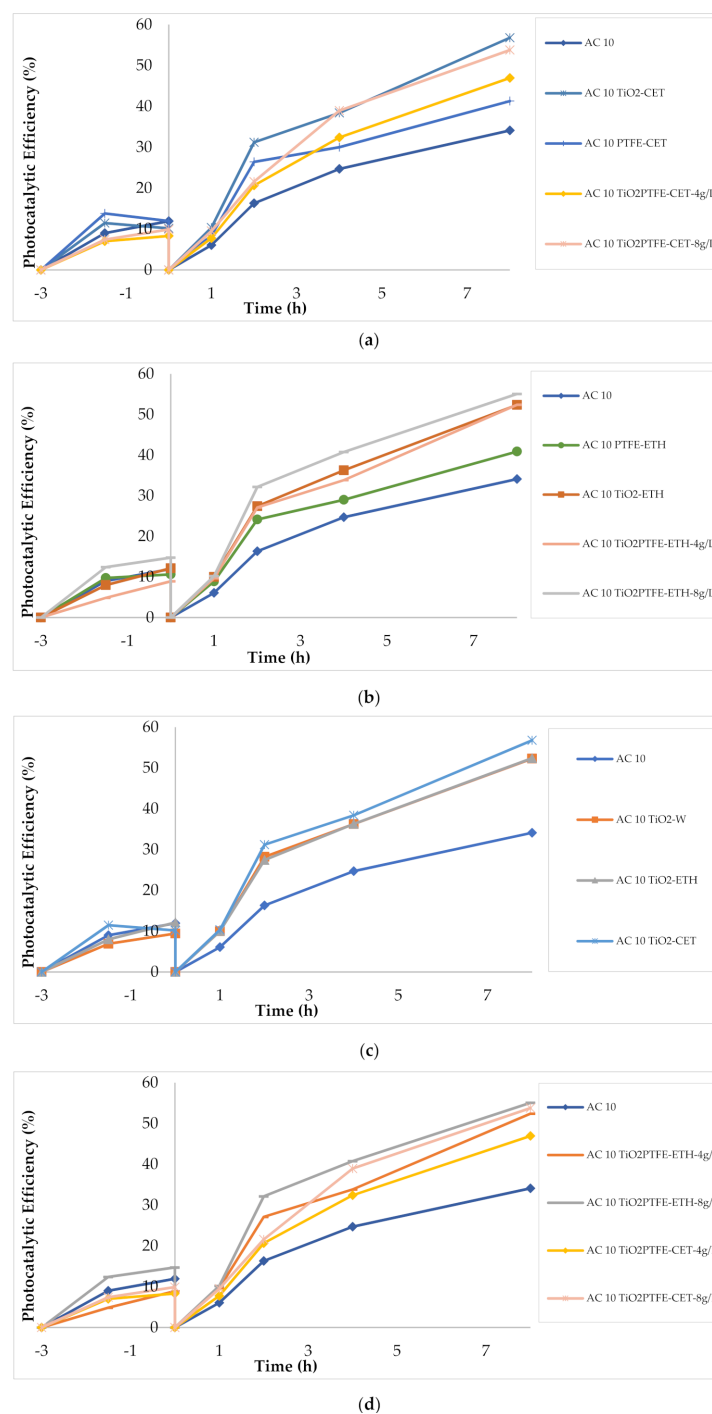
Figure 4. Photocatalytic efficiency of the samples comparing the: (a) particles with ketone; (b) particles with ethyl alcohol; (c) solvent with TiO 2 ; (d) solvent with TiO 2 and PTFE from the first step (selection of best solution).
