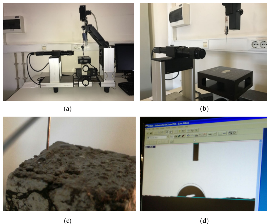
Figure 2. Water contact angle test: (a,b) OCA 15 plus Dataphysics; (c) detail of the water drop over the asphalt mixture samples; and (d) detail of the water drop image in the software.
