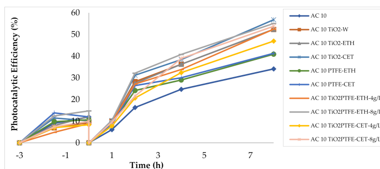
Figure 3. Photocatalytic efficiency of all the samples from the first step (selection of best solution).
