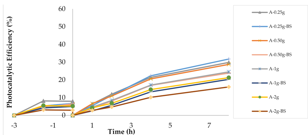
Figure 10. Results of photocatalytic efficiency of the Mixture A with resin and BS.
