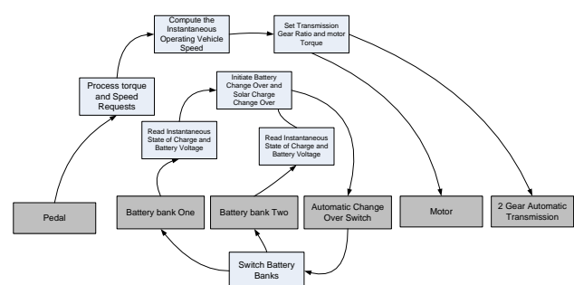
Figure 7: Power Train High Level Control Requirements
