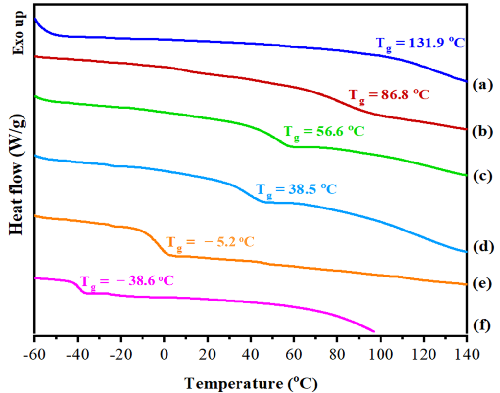
Figure 7. DSC thermogram of CHI (a), their blends (b–e), and P3HPEI (f). Content of P3HPEI in the blends: 20 (b), 40 (c), 60 (d), and 80% (e).
