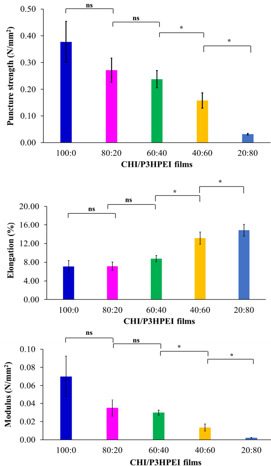
Figure 10. Mechanical properties of CHI and their blends with P3HPEI. Statistically significant differences are given as: *— p < 0.05 ; ns—no significance.
