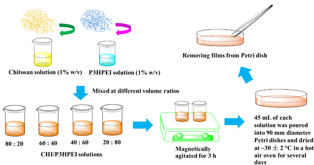
Figure 1. Scheme of CHI/P3HPEI films preparation.
