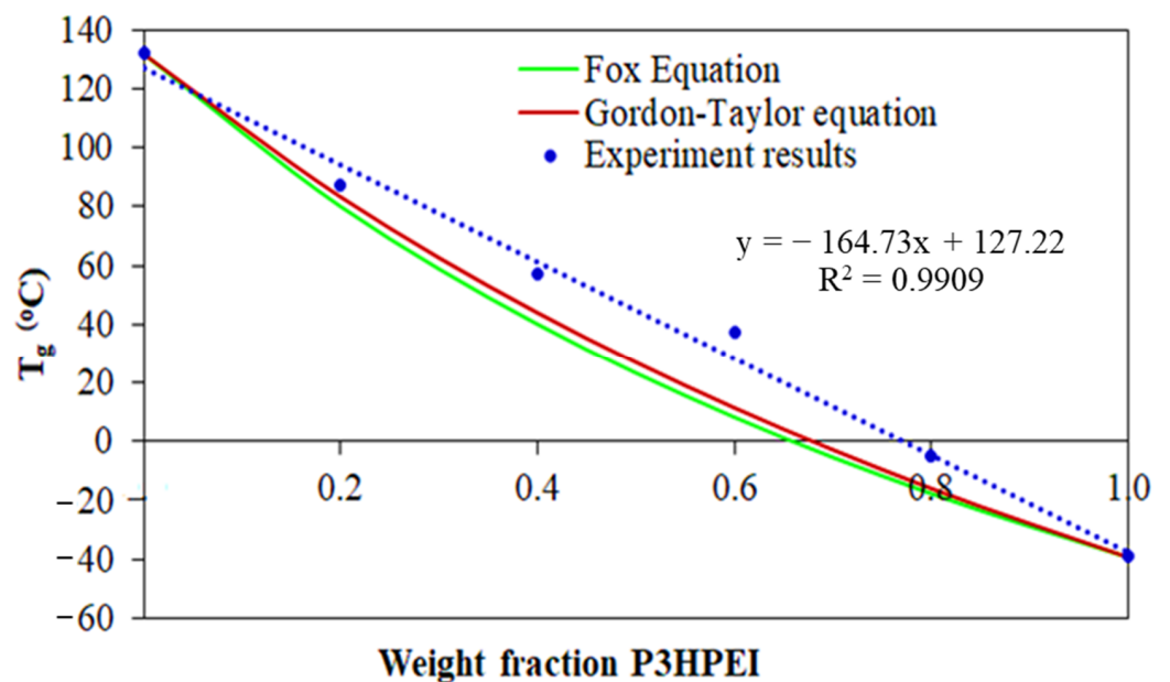
Figure 8. Correlation between weight fraction of P3HPEI and T_g of experimental results, compared with theoretical results.
