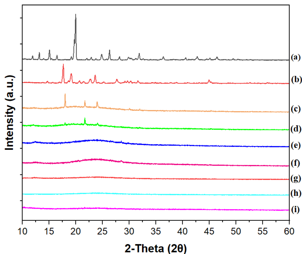
Figure 11. XRD diffractograms of haloperidol (a), haloperidol HCl (b), CHI/P3HPEI films loaded with haloperidol at various% drug loading, 5.0% (c), 2.5% (d), 2.0% (e), 1.75% (f), 1.5% (g), and 1.25% HP films (h) and drug-free CHI/P3HPEI film (i).
