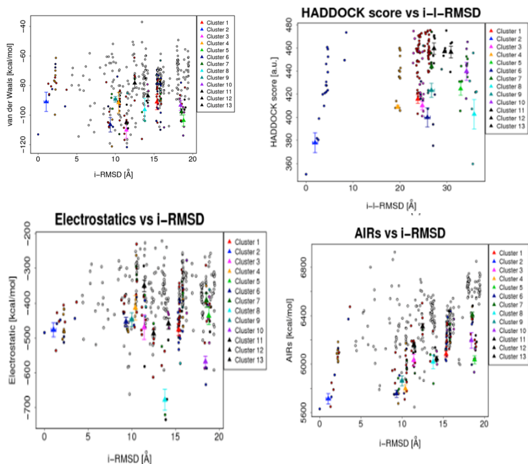
Clusters of NS3/4A- V H H24
