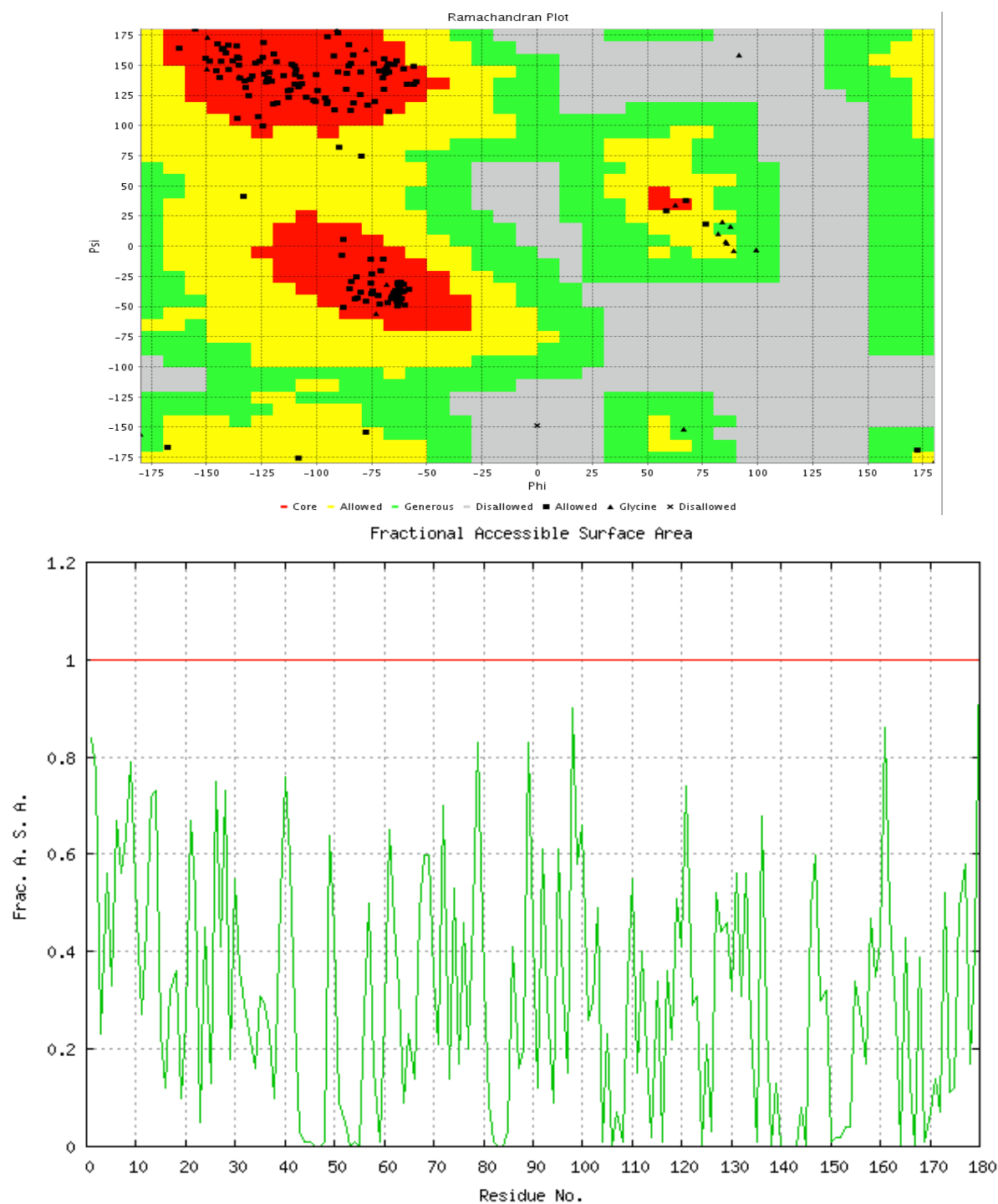
Supplemental data 1. The quality criteria of the NS3/4A models.
