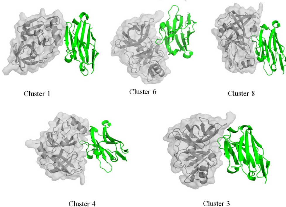
Clusters of NS3/4A- V H H24
