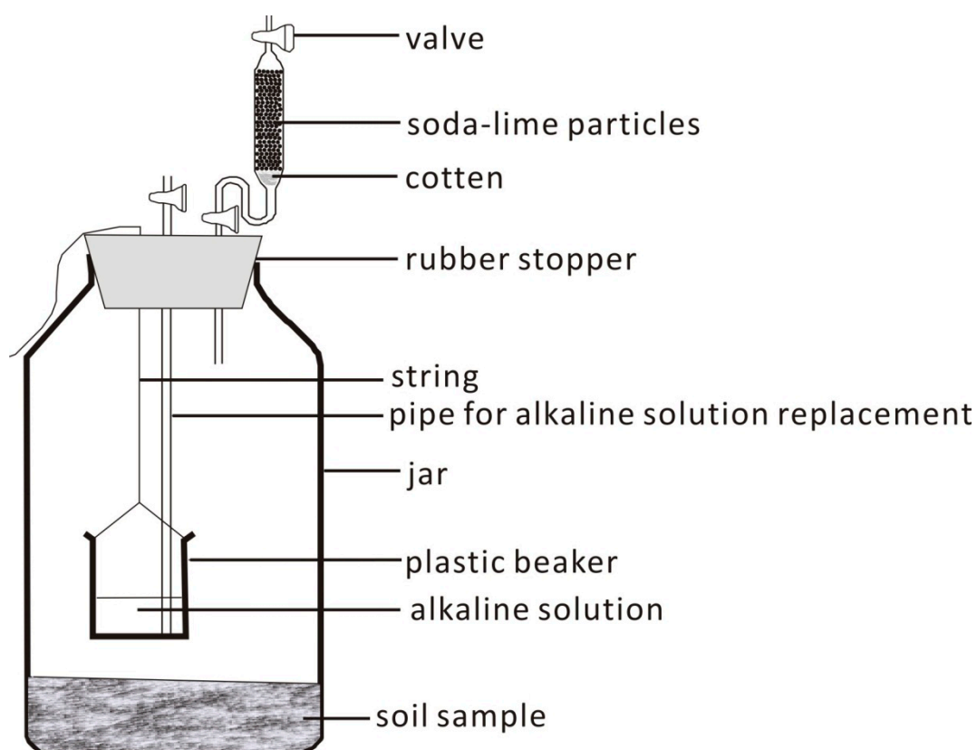
Figure S2. The sketch of incubation device.
