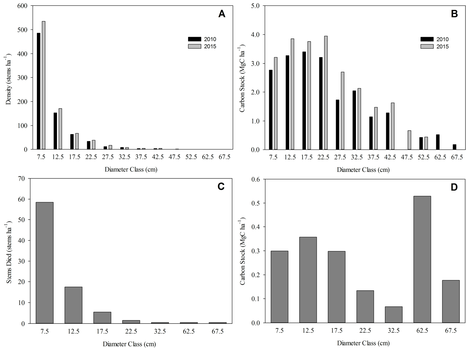
Figure S1. A) Density (stems \text{ha}^{-1} ) of live trees; B) Carbon Stock ( \text{MgC ha}^{-1} ) of live trees; C) Stems died (stems \text{ha}^{-1} ) in the period 2010-2015; and D) Carbon Stock ( \text{MgC ha}^{-1} ) of dead trees in the period 2010-2015.
