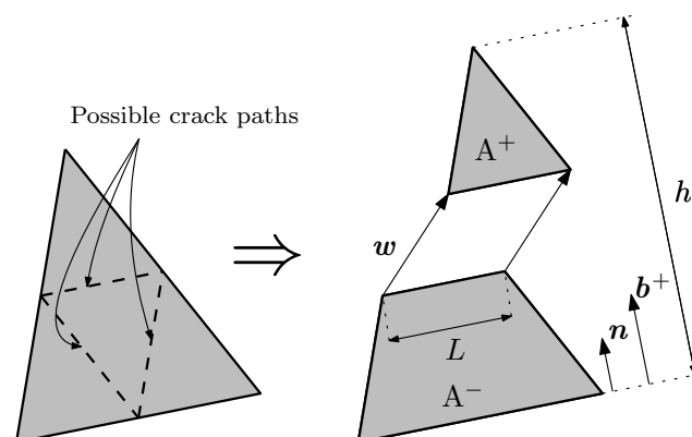
Figure 3. Embedded cohesive crack element.
