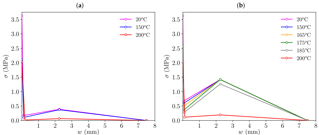
Figure 6. Trilinear softening diagrams used for simulating PFRC fracture specimens subjected to different high-temperature conditions: (a) HF3 specimens, (b) HF10 specimens
