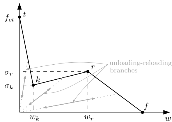
Figure 4. Trilinear softening diagram used to reproduce fracture in PFRF.
