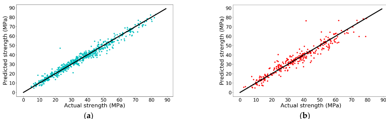
Figure 9. Prediction accuracy of XGBoost: (a) training set and (b) test set.
