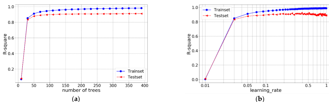
Figure 7. R-square of XGBoost under different hyperparameters: (a) different n\_estimators ; and (b) different learning rate.
