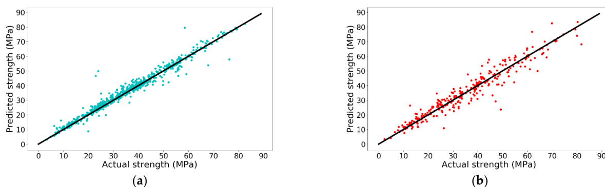
Figure 14. Prediction accuracy of ANN with different neurons in each layer: (a) training set and (b) test set.
