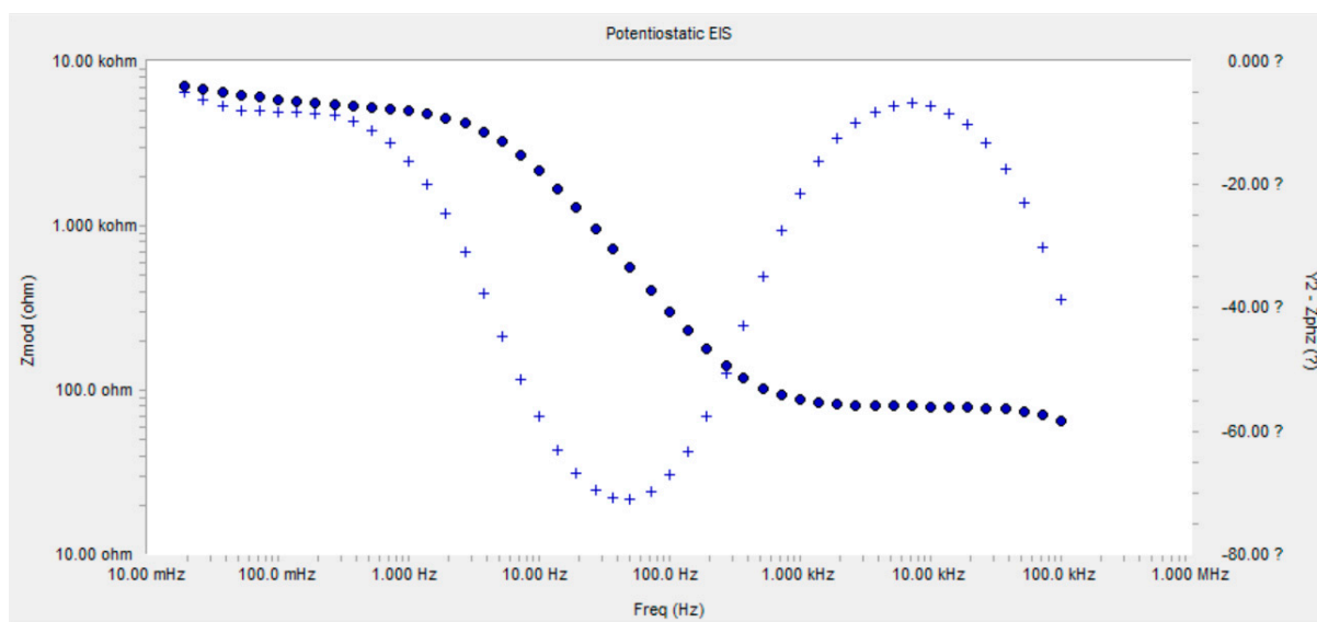
Figure S2. Bode Plot for 1 mM Selenite.
