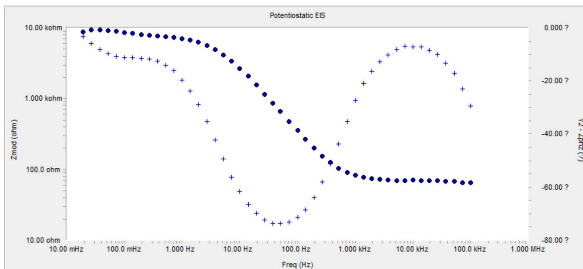
Figure S4. Bode Plot for 10 mM Selenite.
