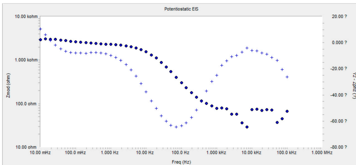
Figure S1. Bode plot for control.
