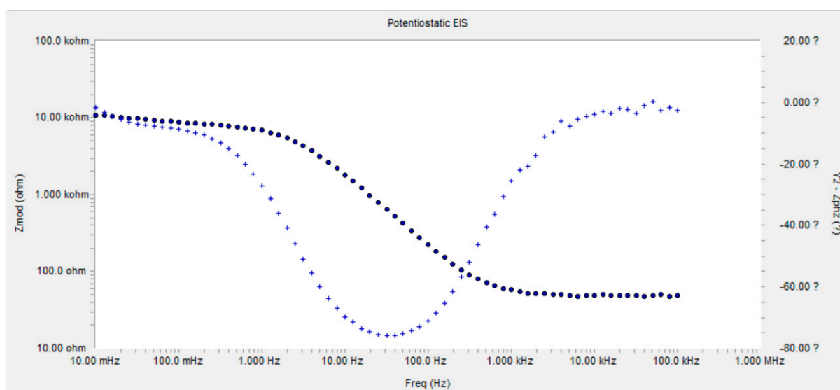
Figure S3. Bode Plot for 5 mM Selenite.
