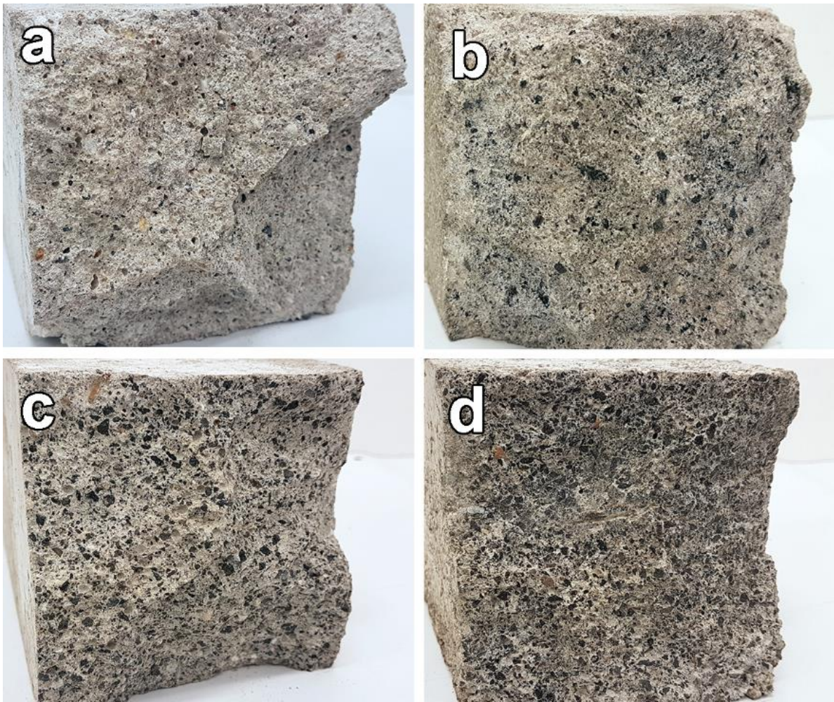
Fig. S1: The collection of prepared prismatic concrete samples with dimensions of 100 x 100 x 400 mm of after flexural strength measurements: a – RC, b – RA-C 10, c – RA-C 50, d – RA-C 100.
