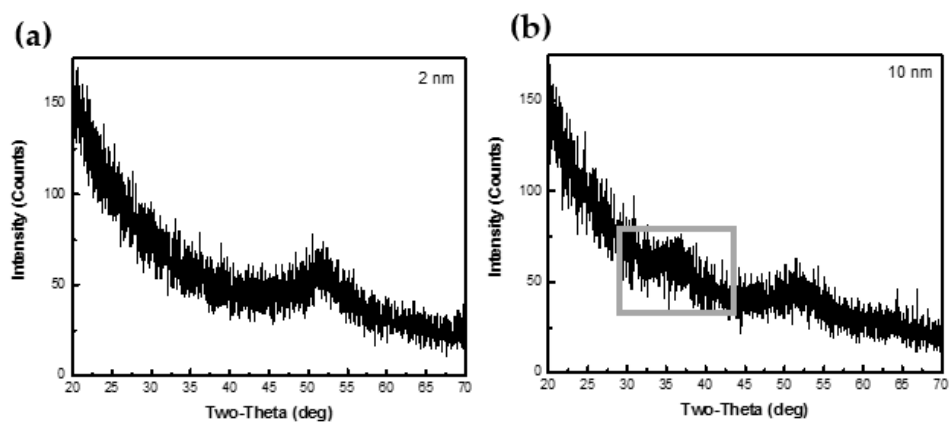
Supporting Figure S1. GIXRD spectra of (a) 2 nm, (b) 10 nm Ti after 250°C 50min oxidation
