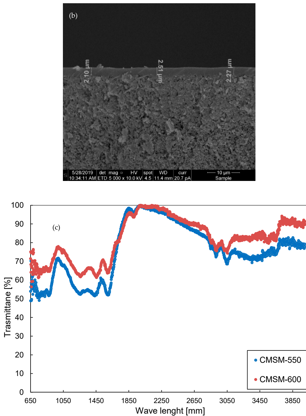
Figure 3. Scanning electron microscopy of CMSM-550: (a) top section of the membrane (b) bottom section of the membrane. (c) Fourier transform infrared (FTIR) of CMSM-550 and CMSM-600.
