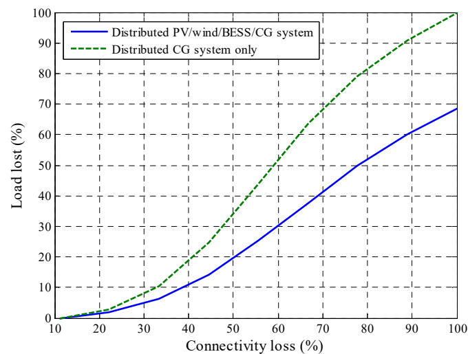
Figure 31. Vulnerability evaluation. (Distributed CG system under CIC).
