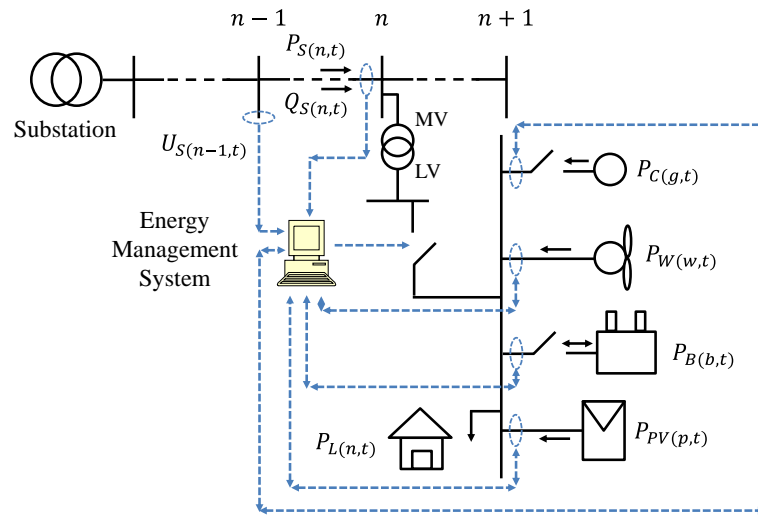
Figure 5. MG structure.
