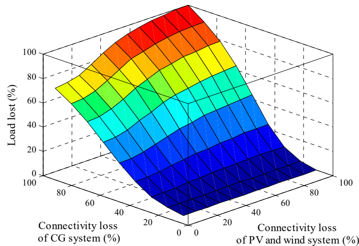
Figure 32. Vulnerability evaluation. (Distributed renewable and CG systems under CIC).
