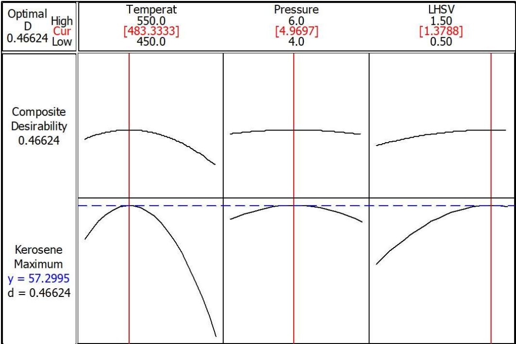
Figure S3. Optimal plot of kerosene selectivity.
