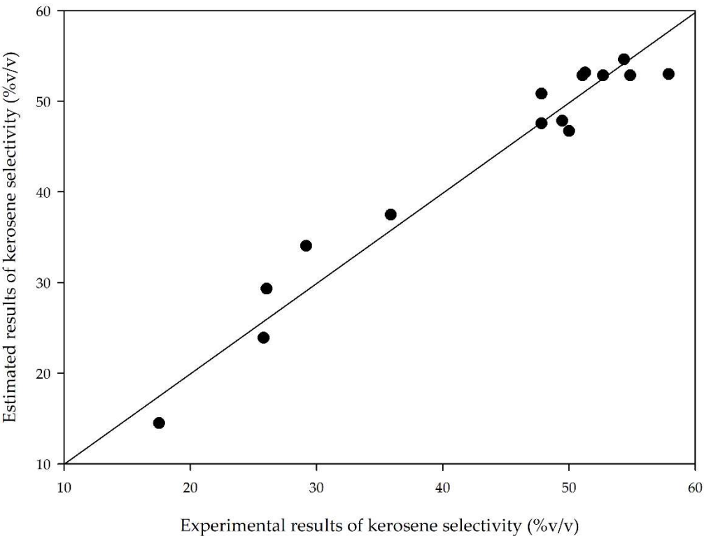
Figure S2. Experimental and estimated results for kerosene selectivity.
