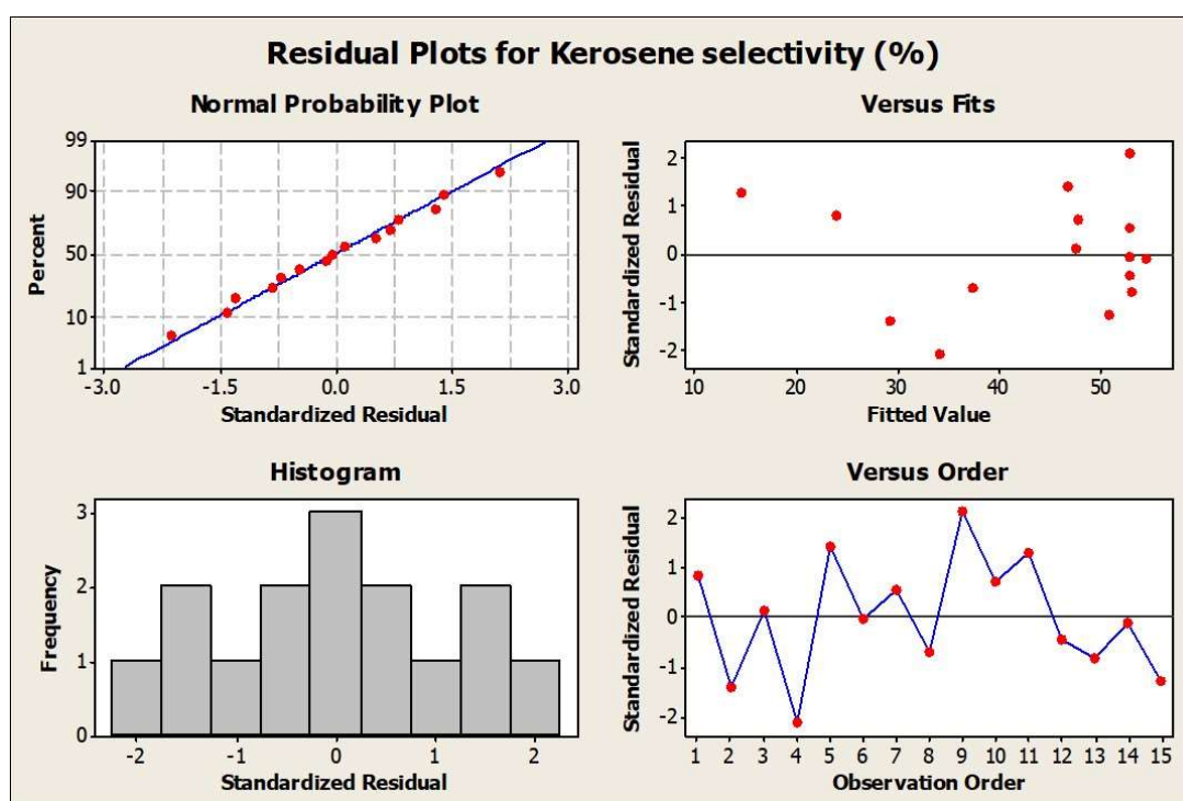
Figure S1. Residual plots of kerosene selectivity.
