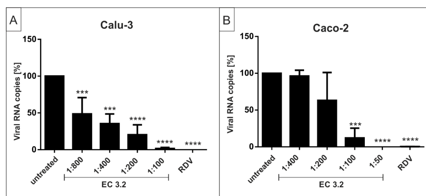
Figure 3. Liquid European black elderberry (EC 3.2) extract inhibits replication of SARS-CoV-2 Wuhan type in Calu-3 and Caco-2 cells. Calu-3 (A) and Caco-2 cells (B) were infected with the clinical isolate SARS-CoV-2 PR-1 at a MOI of 2 \times 10^{-2} . One hour after infection and removal of input virus, cells were treated with indicated dilution steps of EC 3.2. A total of 1 \mu M Remdesivir (RDV) was included as a positive control. Cell culture supernatants were harvested at 3 dpi. The virions were purified and analyzed by qRT-PCR. Bars show mean values of three independent experiments \pm standard deviation. Statistical analysis was performed using a multiple comparison Kruskal–Wallis test (Anova) followed by Dunn’s post hoc test (***) p < 0.001 ; **** p < 0.0001 versus the untreated control).
