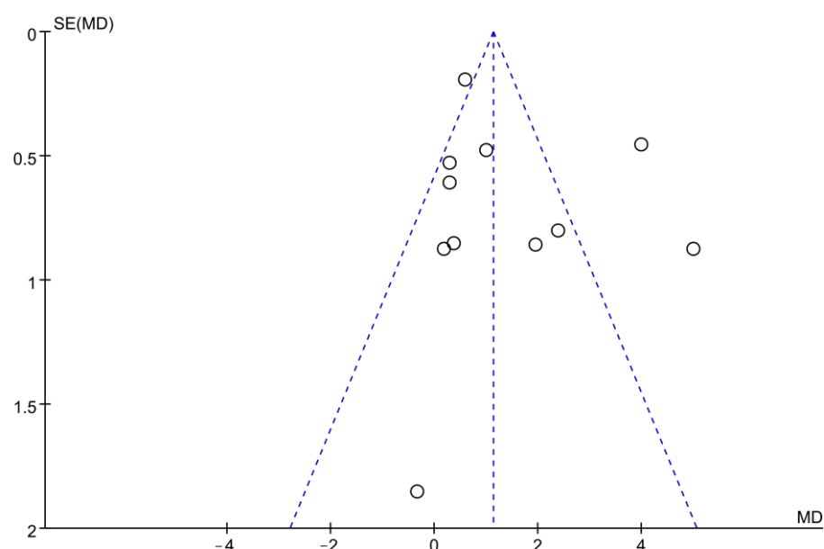
Figure 3. Funnel plot.
