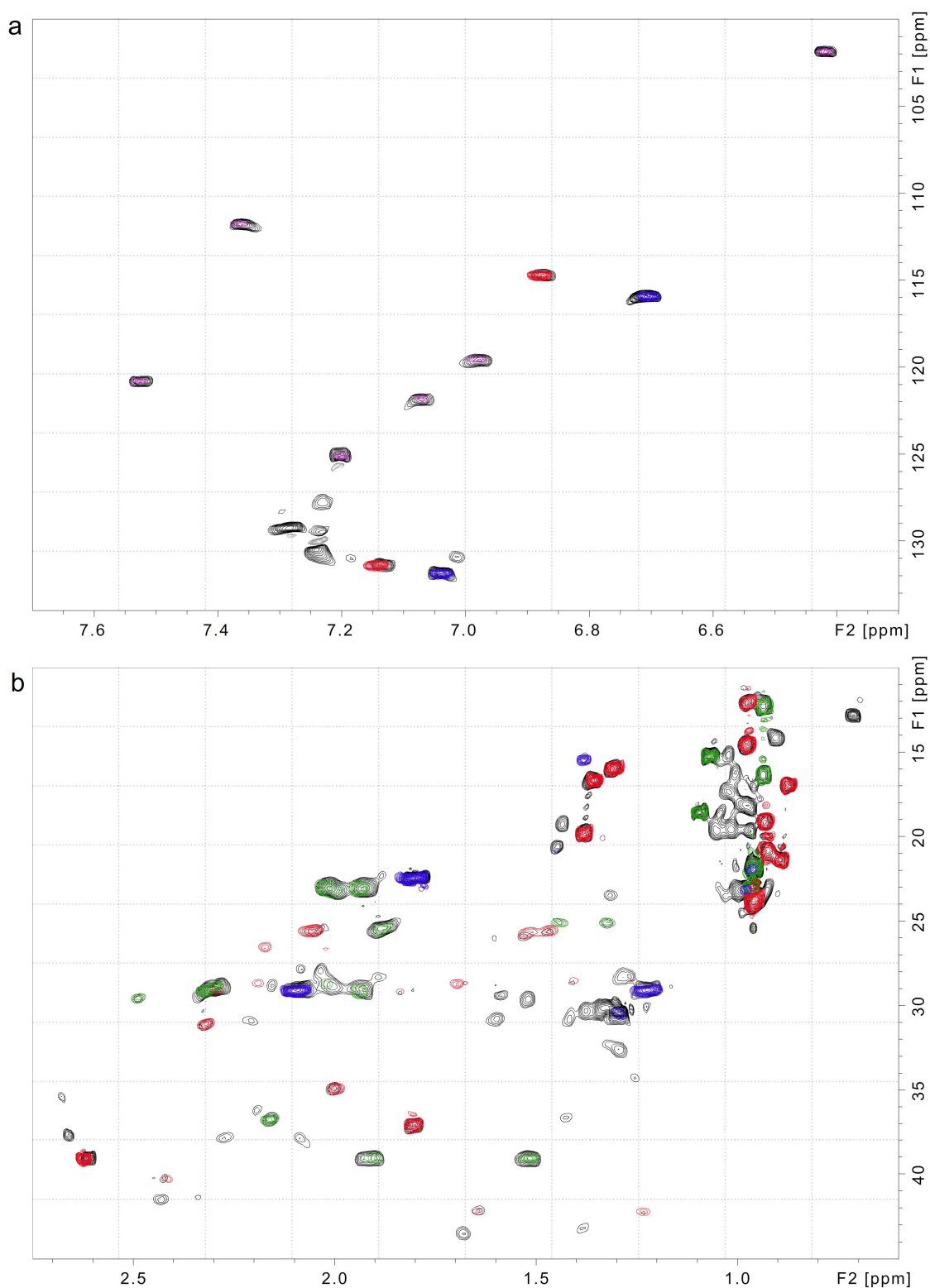
Figure 3. Atomic Sort identification of didemnin B (1) in the T. mobilis JCM21370. Expansions of (a) the aromatic and (b) the methyl regions of the ^1\text{H} - ^{13}\text{C} HSQC spectrum of the T. mobilis JCM21370 extract H (black) overlaid with spectra of didemnin B (1, red), cyclo(Pro-Tyr) (3, blue), Leu-Pro-Ile-Pro-Ile (2, green), and indole (magenta). All peaks of these metabolites are observed in the T. mobilis JCM21370 extract spectrum, along with additional weaker peaks from metabolites that were not identified. Extract H (Table 2) was used for this study.
