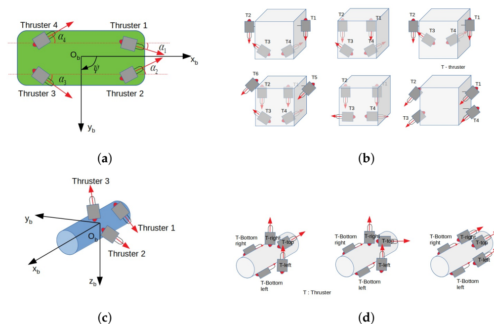
Figure 16. Different reconfigurable underwater robots. (a) Tortuga robot's configuration. (b) e-URoPe robot's configuration. (c) RSM robot's configuration. (d) Amour 6 robot's configuration.
