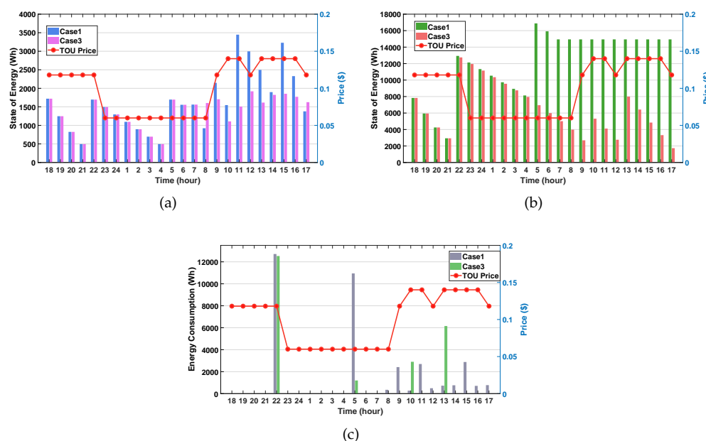
Figure 6. Performance comparison between Case 1 and Case 3. (a) SOE of the ESS; (b) SOE of the EV; (c) net consumption of household.
