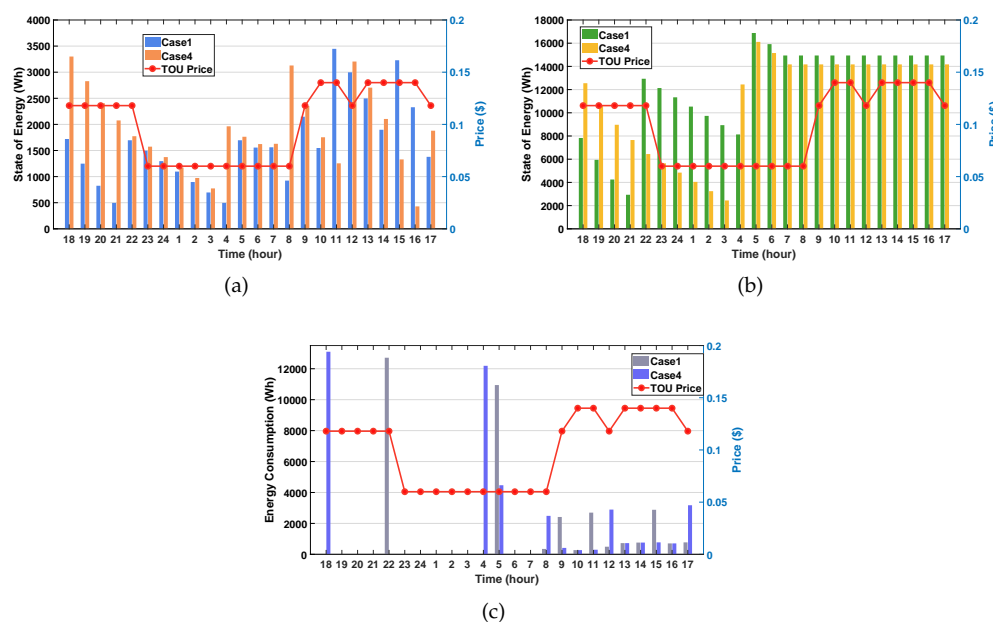
Figure 7. Performance comparison between Case 1 and Case 4. (a) SOE of the ESS; (b) SOE of the EV; (c) net consumption of household.
