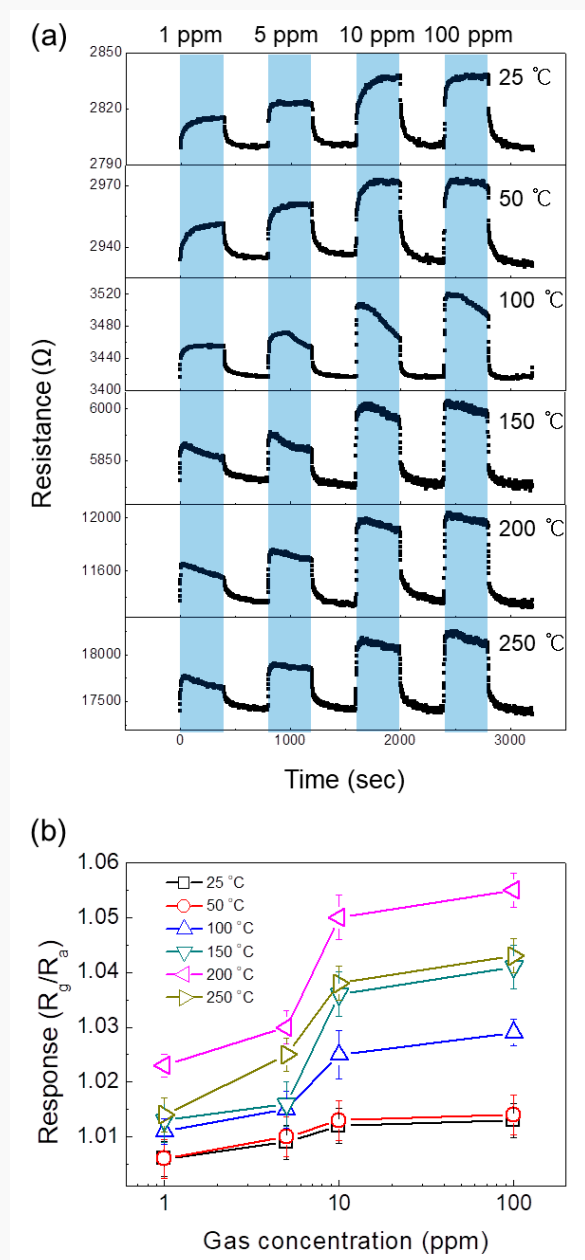
Figure S1. (a) Dynamic resistance curves of the pure Pd gas sensor to various concentrations of H_2 gases at different temperatures. (b) Corresponding calibration curves.
