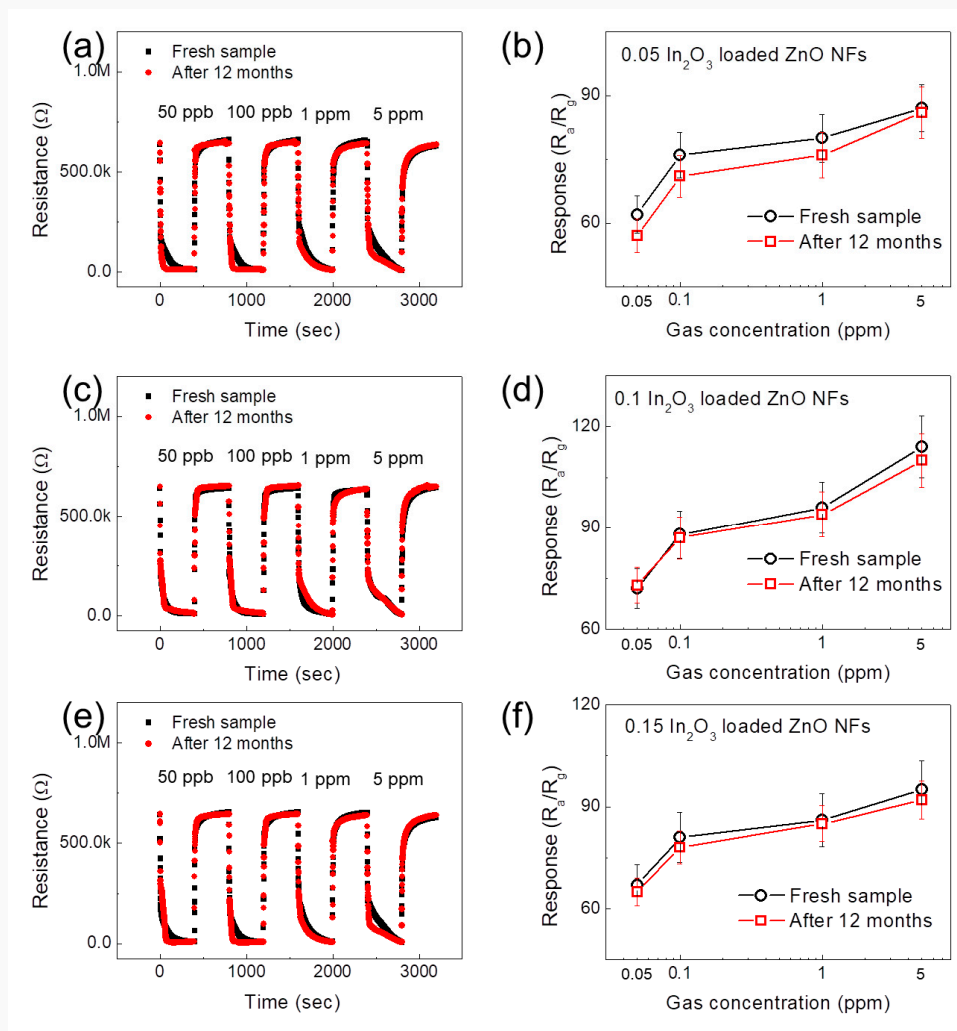
Figure S2. Dynamic resistance curves and corresponding response versus \text{H}_2 gas concentration of the fresh and 12 months aged (a) and (b) 0.05, (c) and (d) 0.1 and (e) and (f) 0.15 \text{In}_2\text{O}_3 -loaded ZnO NFs gas sensors, respectively.
