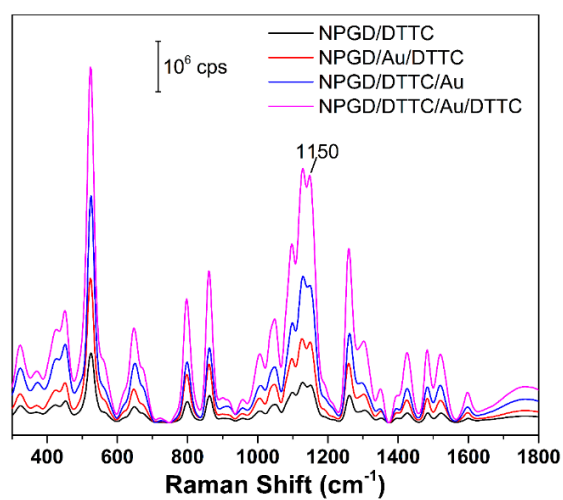
Figure S2. SERS spectra of DTTC on NPGD/13 nm AuNP composites.
