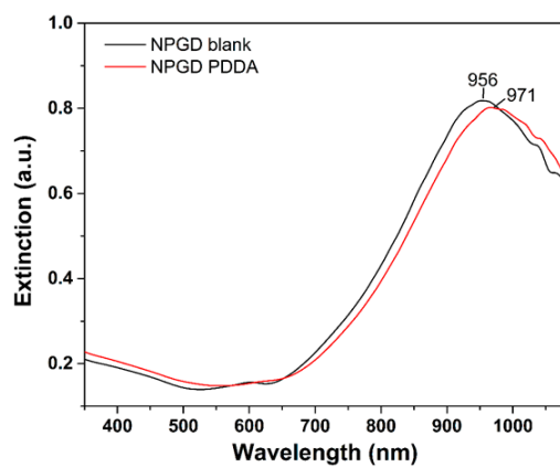
Figure S1. Extinction spectra of NPGD before and after adsorbing PDDA.
