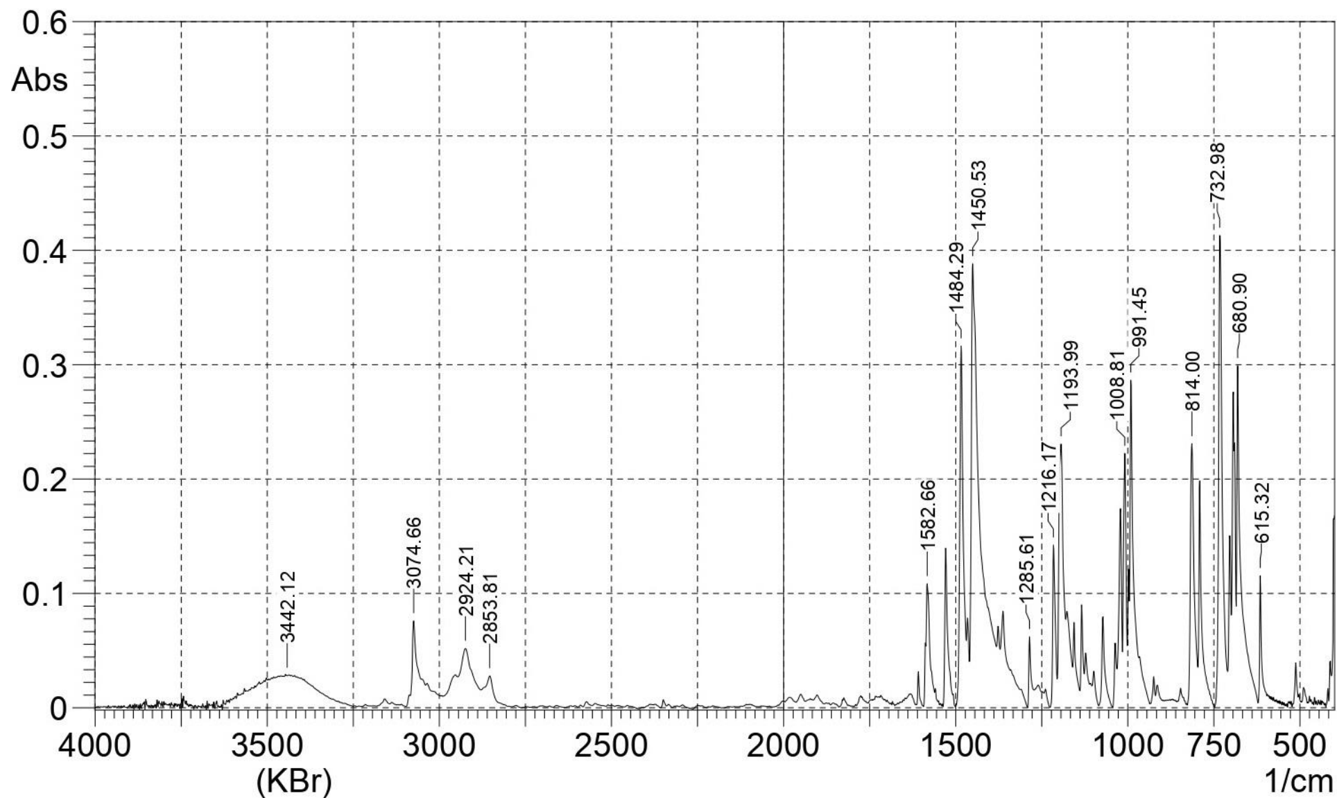
Figure S3. IR spectrum of 3-(5-phenyl-2H-tetrazol-2-yl)-pyridine (in KBr).
