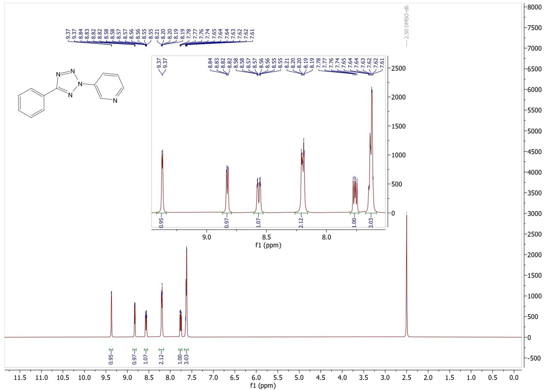
Figure S1. 1 H NMR spectrum of 3-(5-phenyl-2H-tetrazol-2-yl)-pyridine in DMSO-d 6 .
