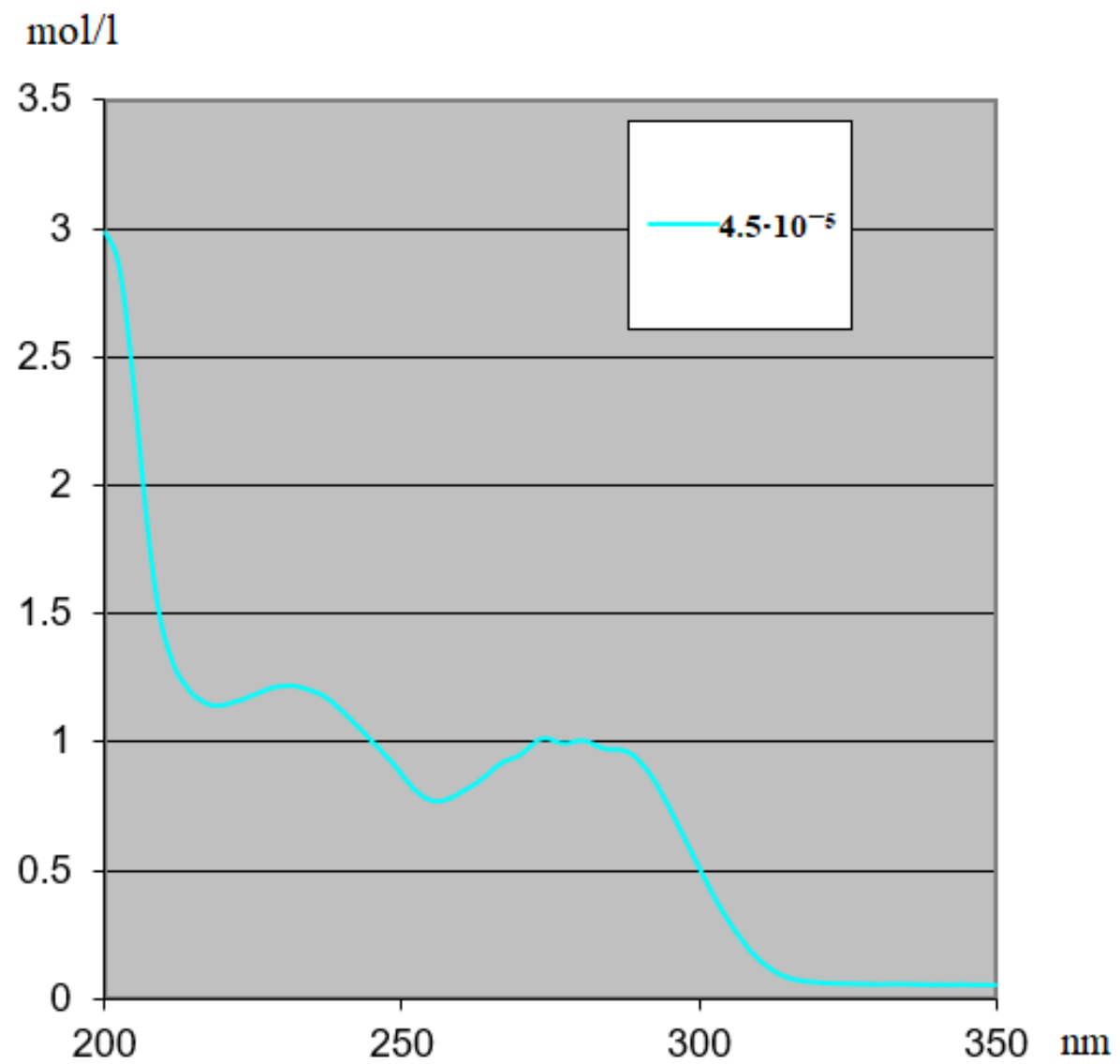
Figure S5. UV-Vis absorption spectrum of 3-(5-phenyl-2 H -tetrazol-2-yl)pyridine 1 .
