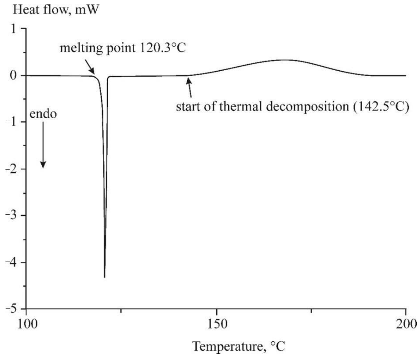
Figure S4. DSC thermogram of 3-(5-phenyl-2 H -tetrazol-2-yl)pyridine 1 .
