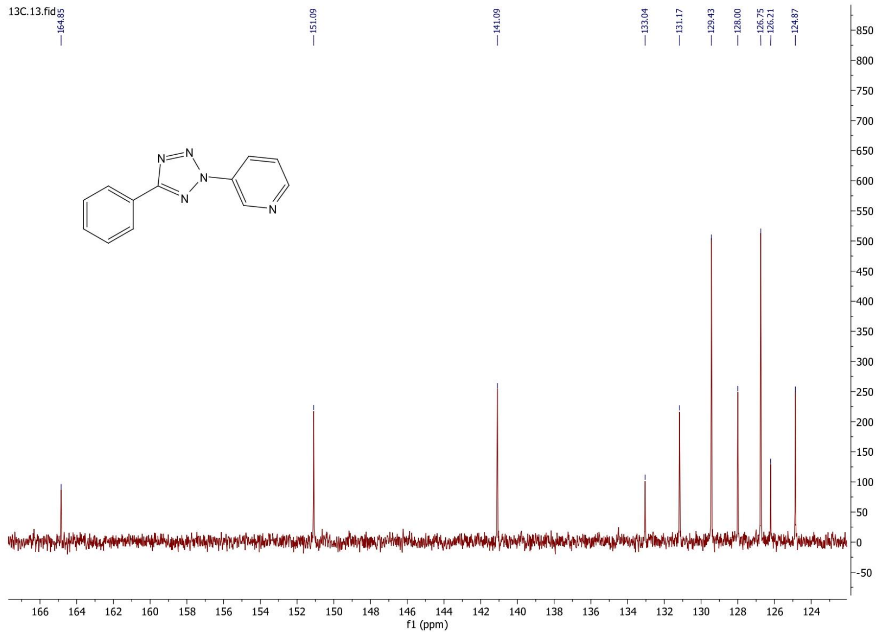
Figure S2. ^{13}\text{C} NMR spectrum of 3-(5-phenyl-2H-tetrazol-2-yl)-pyridine in \text{DMSO-d}_6 .
