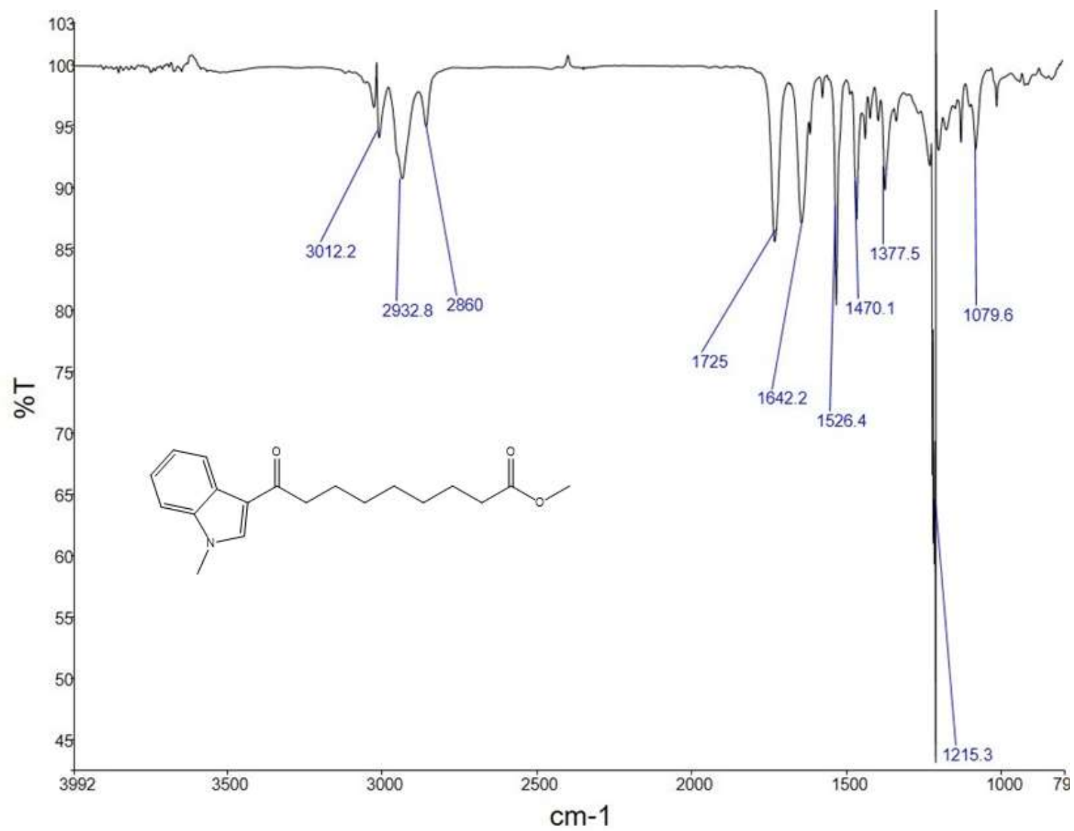
Figure S6. FT-IR spectrum of compound 3 in CDCl 3 .
