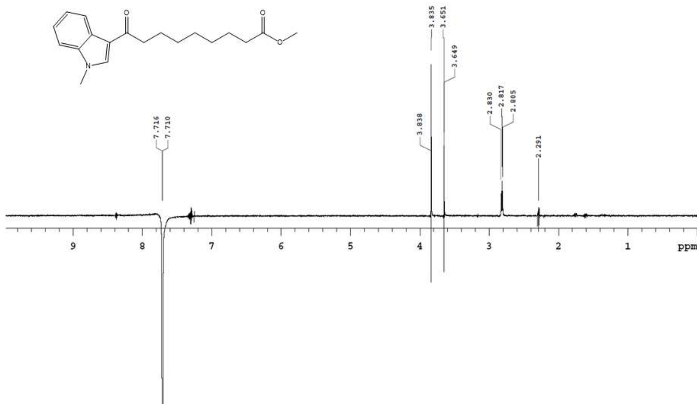
Figure S4. NOE spectrum of compound 3 in \text{CDCl}_3 (Irradiation 7.71 ppm).
