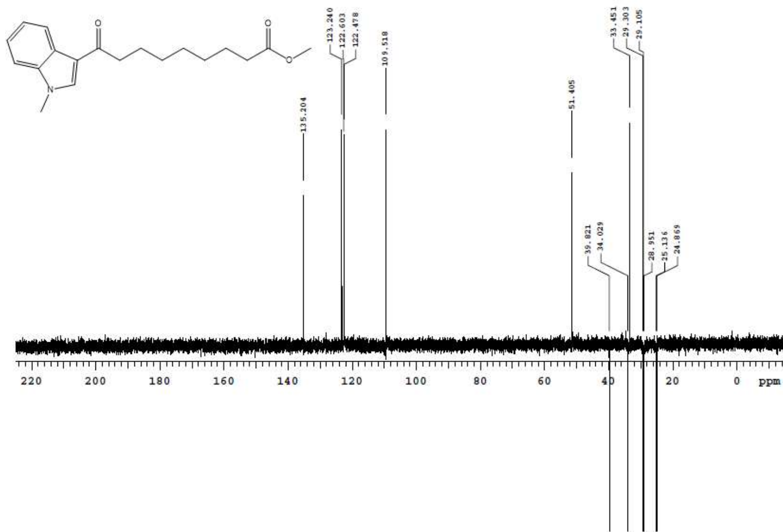
Figure S3. DEPT spectrum of compound 3 in CDCl 3 .
