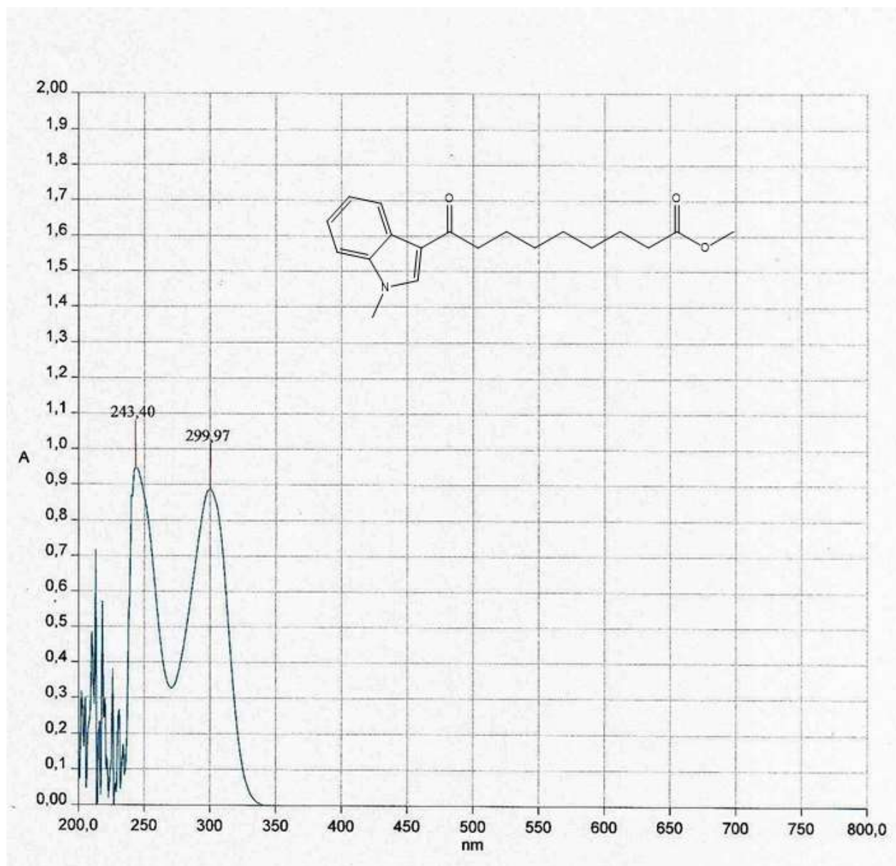
Figure S7. UV-Vis spectrum of compound 3 in \text{CDCl}_3 .
