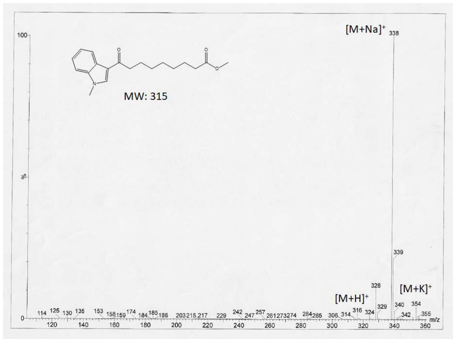
Figure S5. ESI-MS + spectrum of compound 3.
