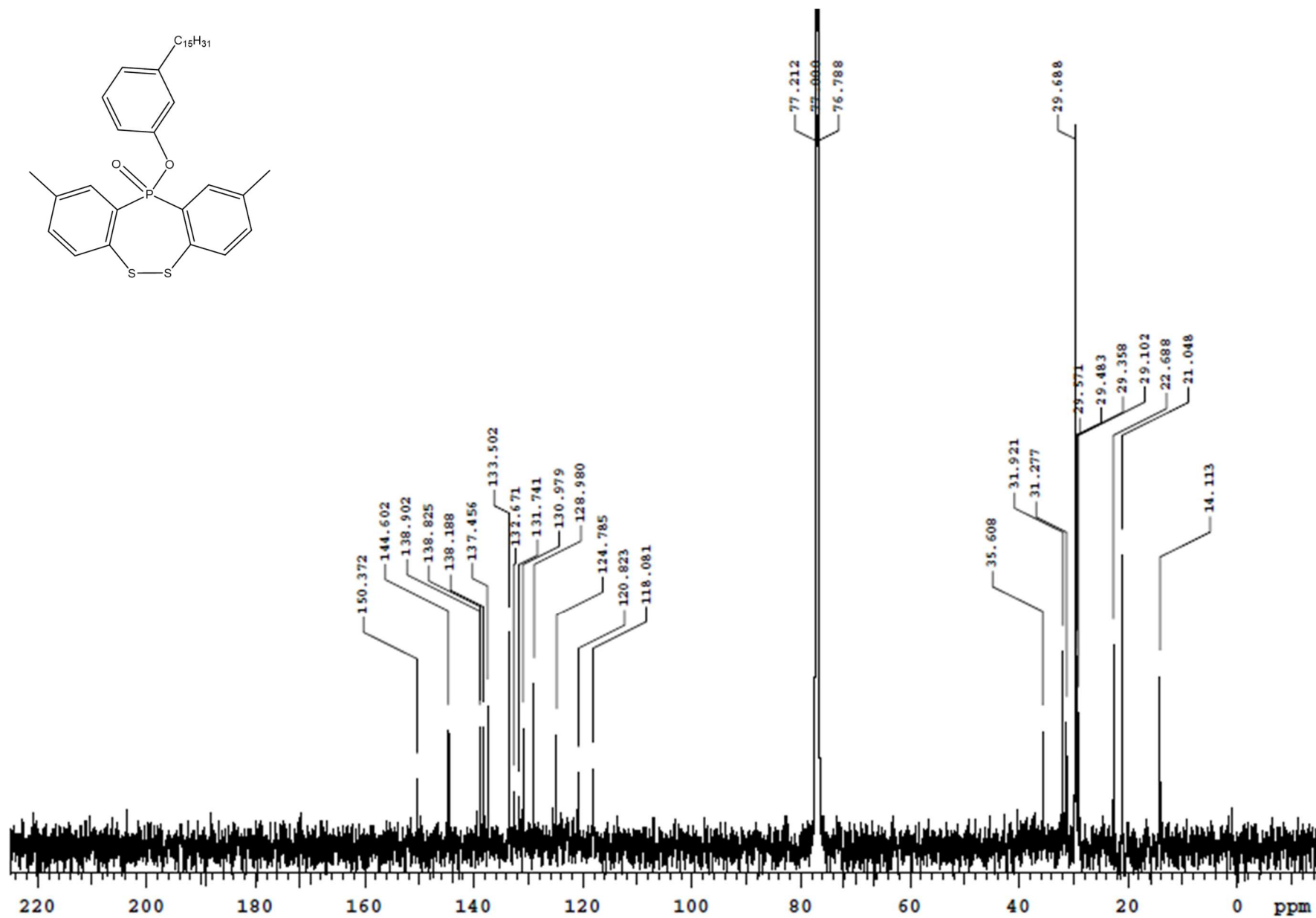
Figure S2: ^{13}\text{C} NMR spectrum in \text{CDCl}_3 of compound 3
