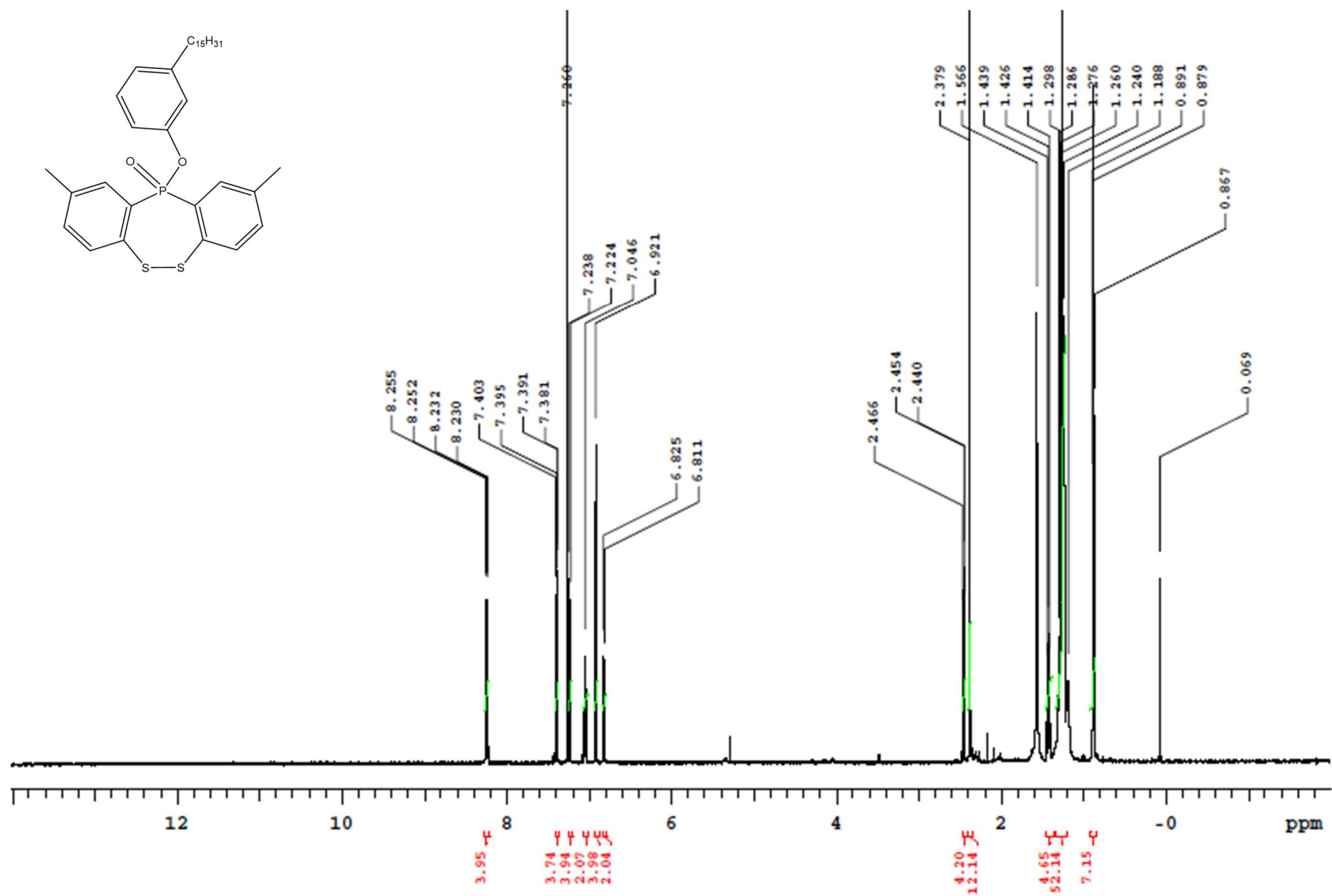
Figure S1: 1 H NMR spectrum in CDCl 3 of compound 3
