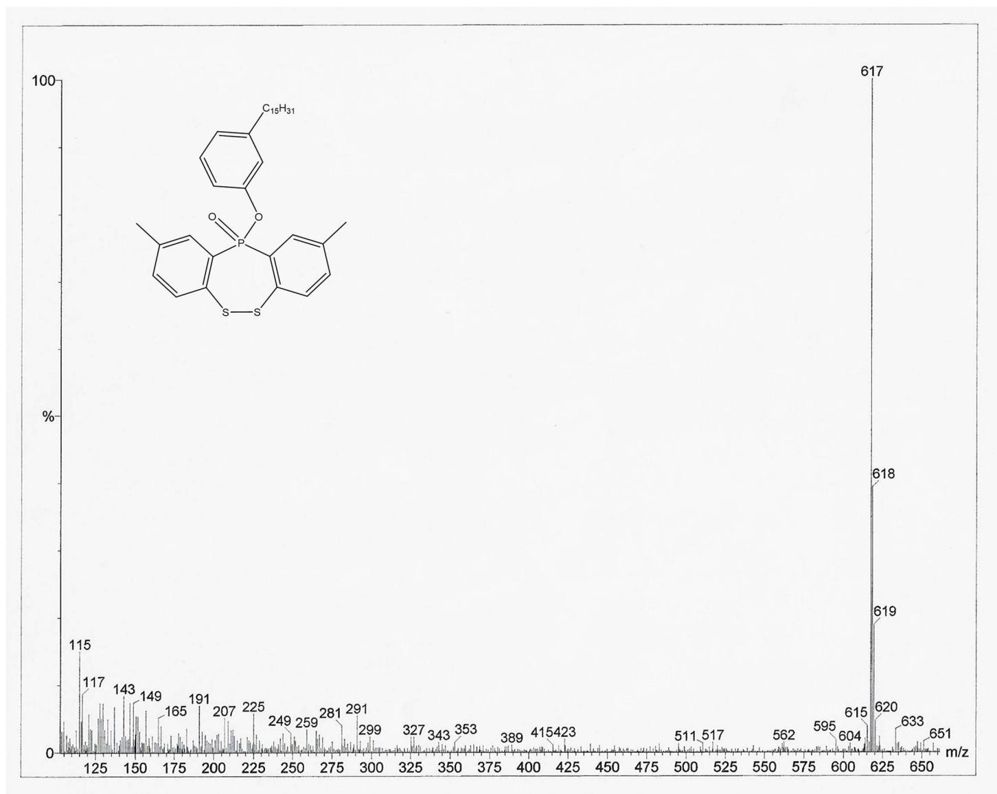
Figure S5: ESI-MS spectrum of compound 3
