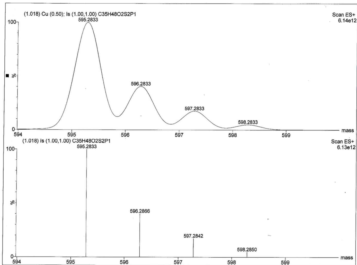
Figure S6: ESI-HRMS spectrum of compound 3
