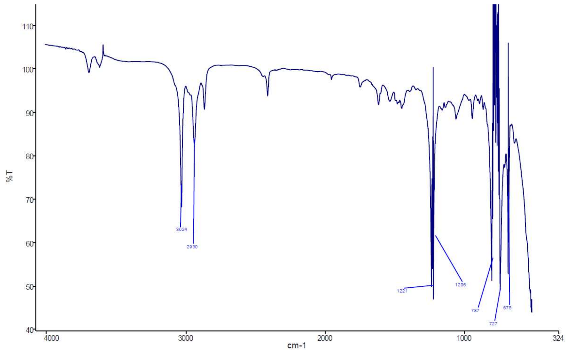
Figure S7: IR spectrum of compound 3
