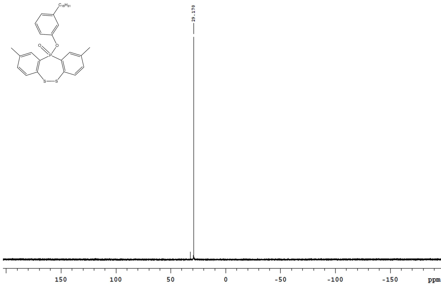
Figure S3: ^{31}\text{P} NMR spectrum in \text{CDCl}_3 of compound 3
