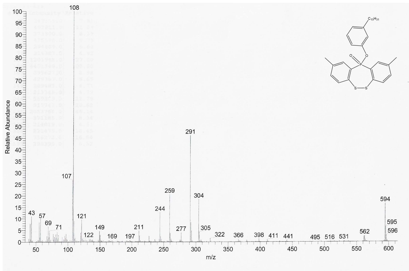
Figure S4: GC-MS spectrum of compound 3
