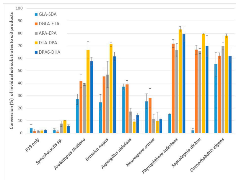
Supplementary Figure S1. Summary of \omega 3D enzymatic activities with the supplied \omega 6 fatty acid salt substrates. \omega 3D activities are shown as conversion rates determined by the amounts of \omega 3 fatty acid products produced from the total amount of \omega 6 fatty acid substrates. Activity from the p19-only control represents the leaf endogenous \omega 3D activity. The error bars denote standard deviations of the means from triplicate assays.
